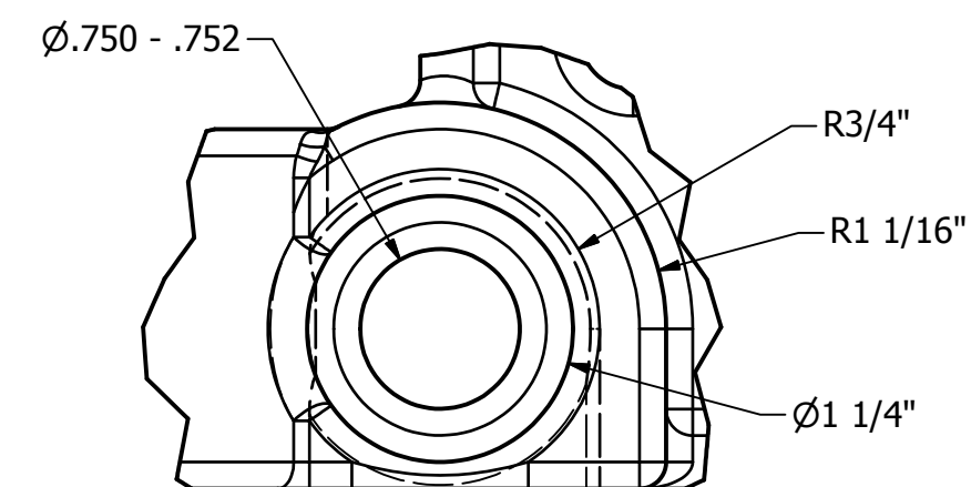
DETAIL E SCALE 1 : 1
