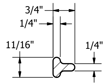
SECTION D-D SCALE 1 / 2
