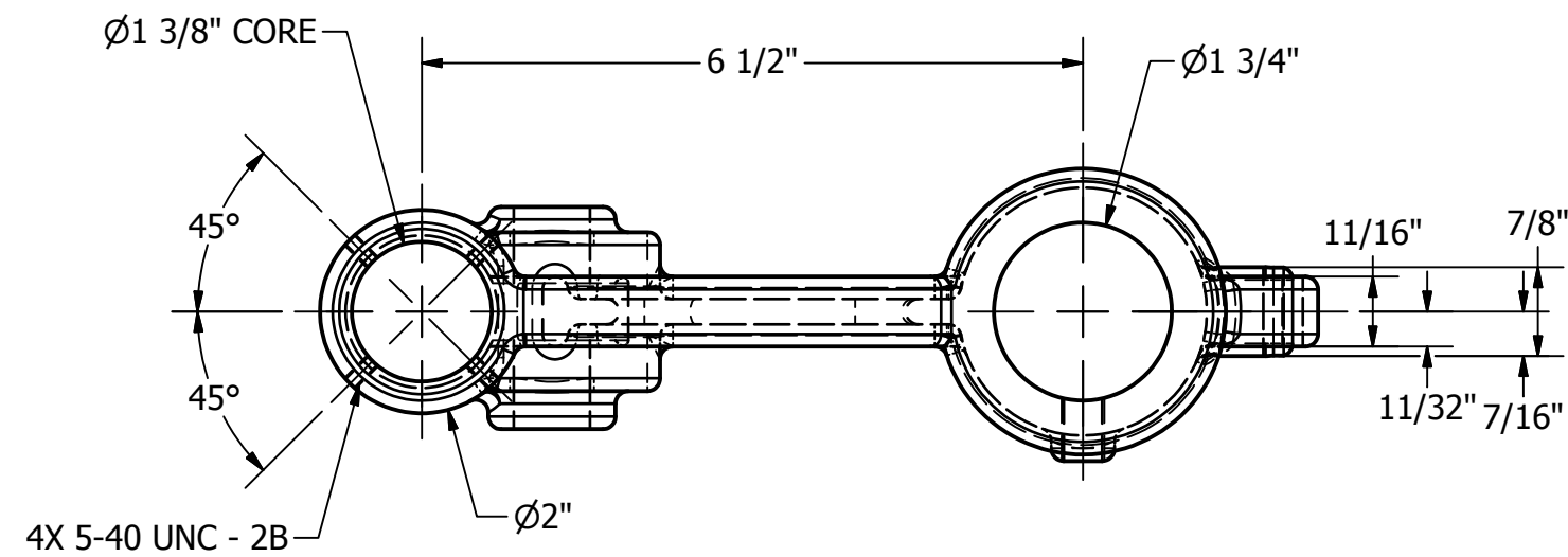
DRILL PRESS BRACKET SCALE 1 / 2
