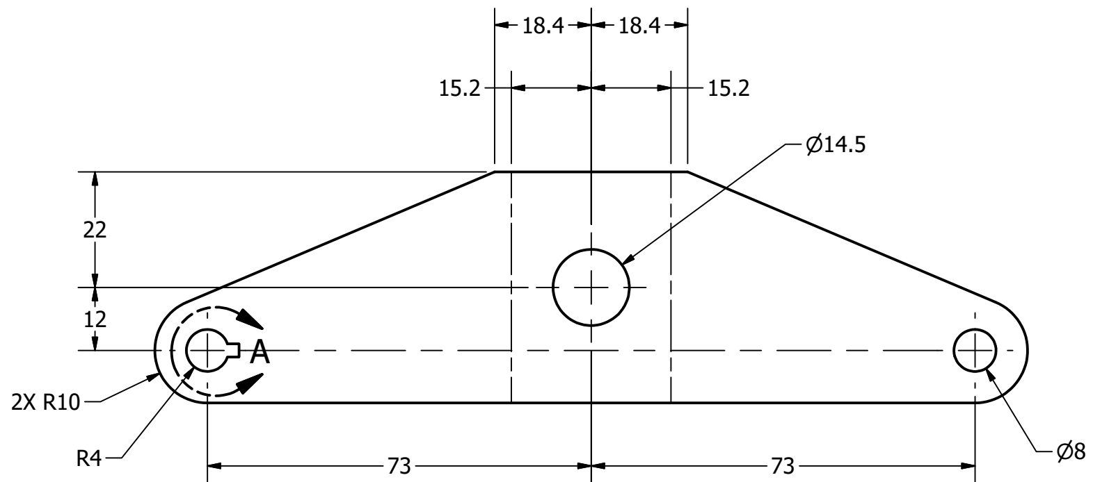
BRACKET FLAT PATTERN SCALE 1 : 1
