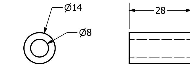
BUSHING SCALE 1 : 1
