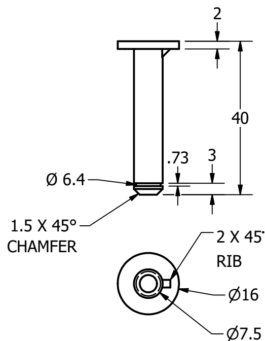
SHAFT SCALE 1 : 1
