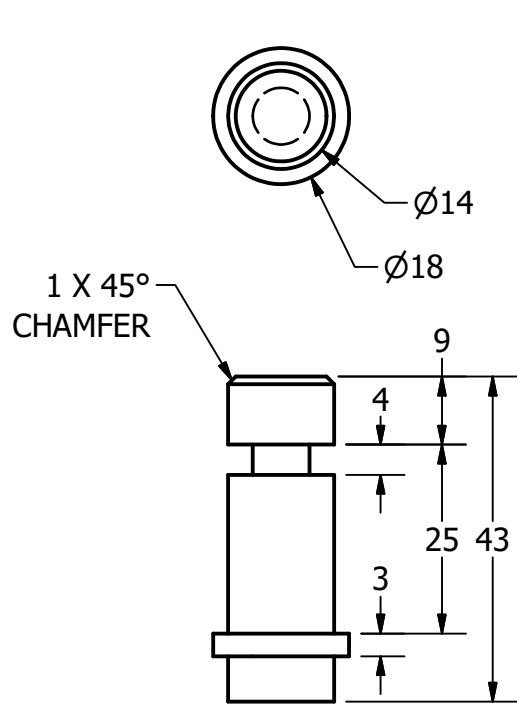
POST SCALE 1 : 1
