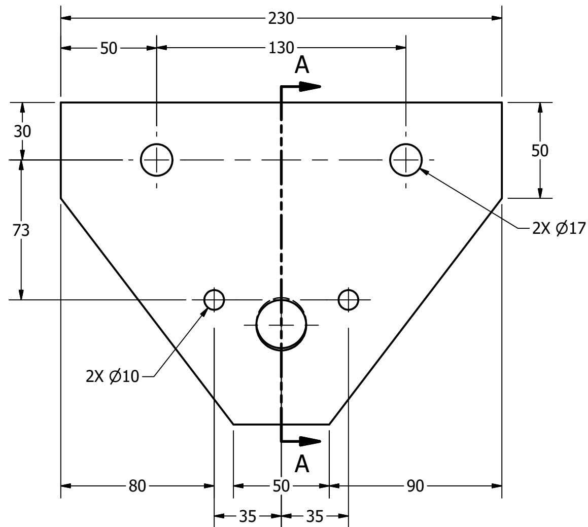
SIDE PLATE SCALE 1 / 2
