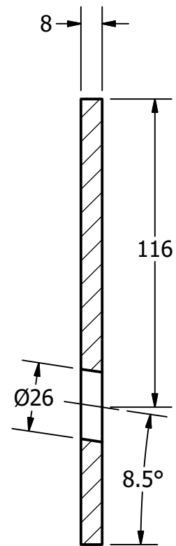
SECTION A-A SCALE 1 / 2
