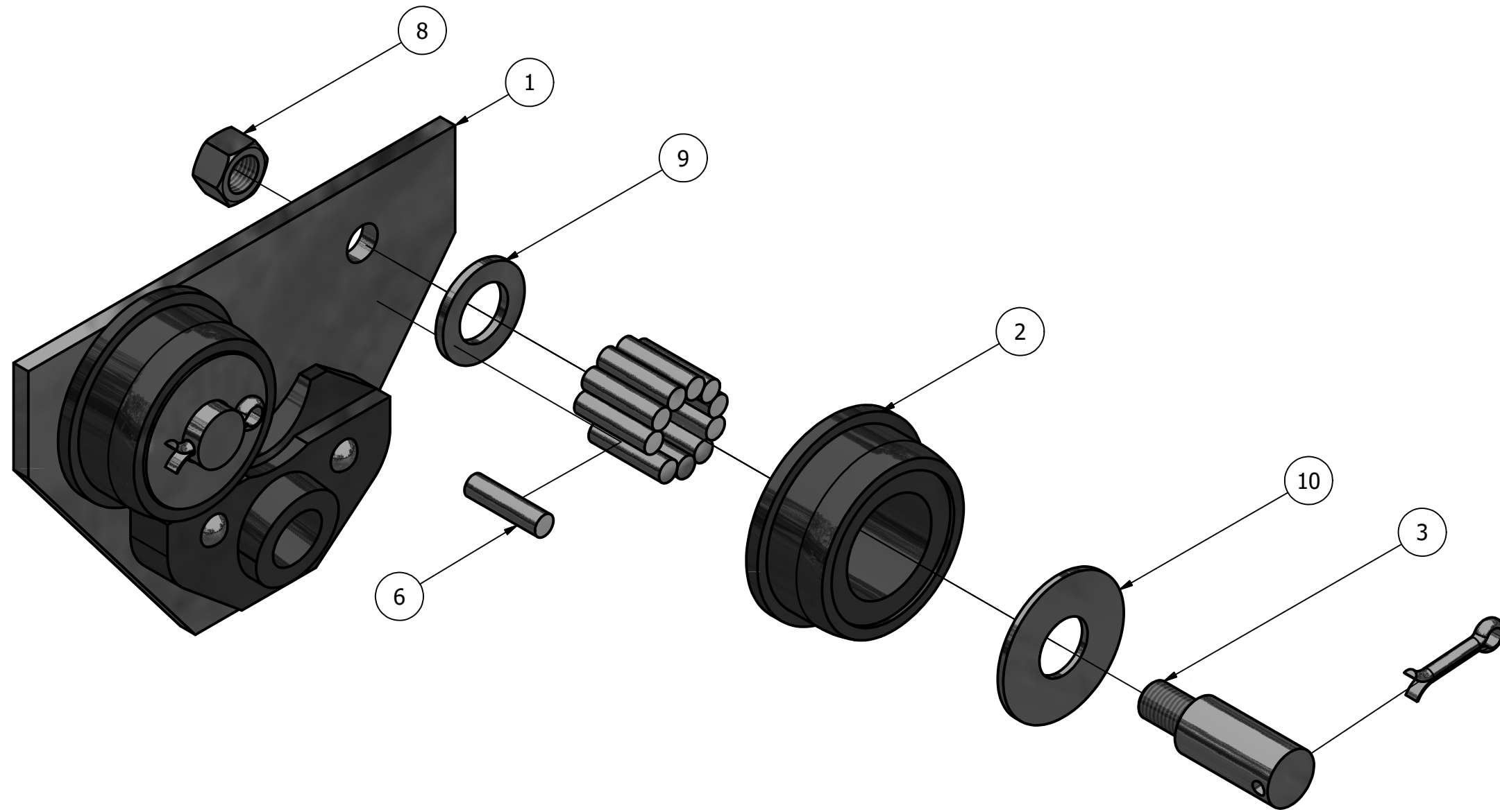
SIDE PLATE EXPLODED ASSEMBLY SCALE 1 / 2
