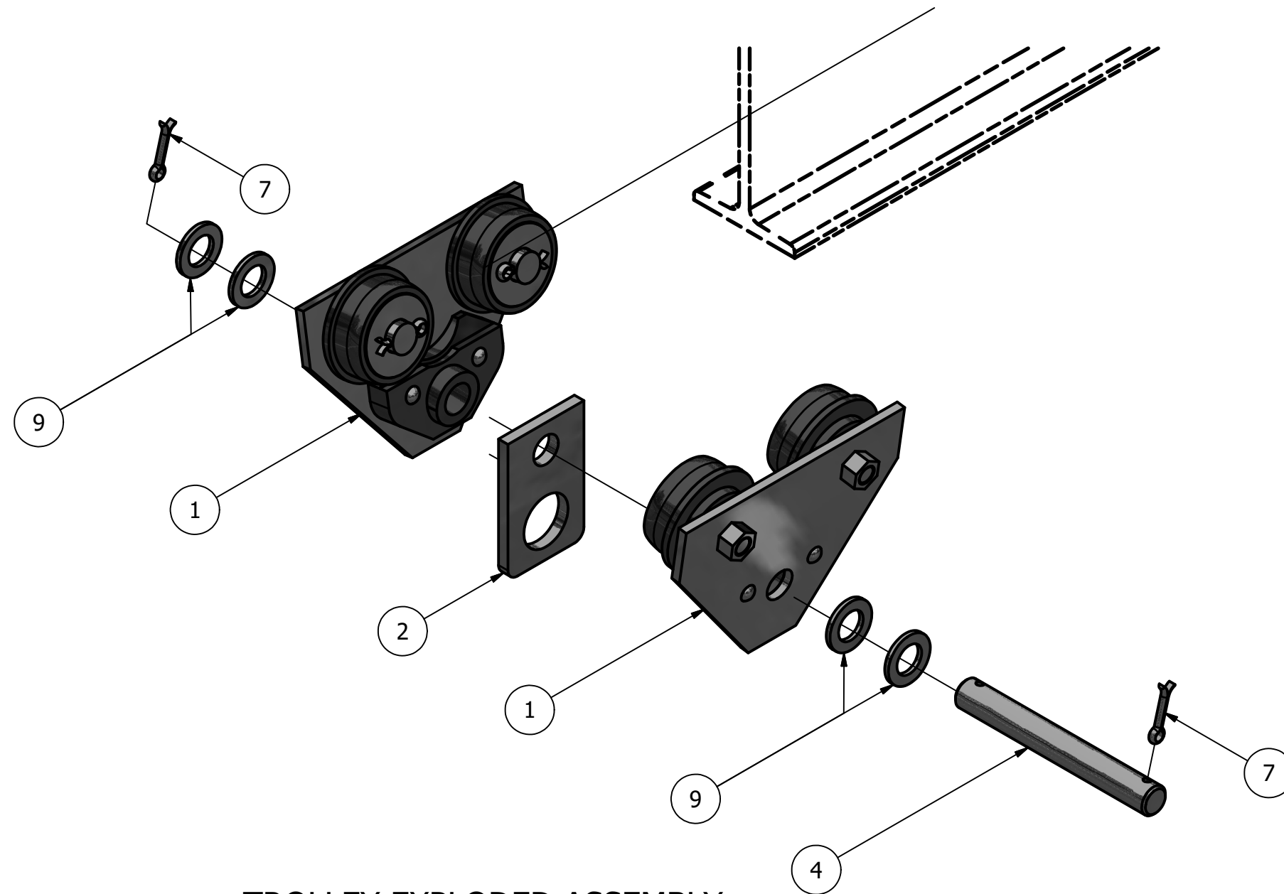
TROLLEY EXPLODED ASSEMBLY SCALE 1 / 4
