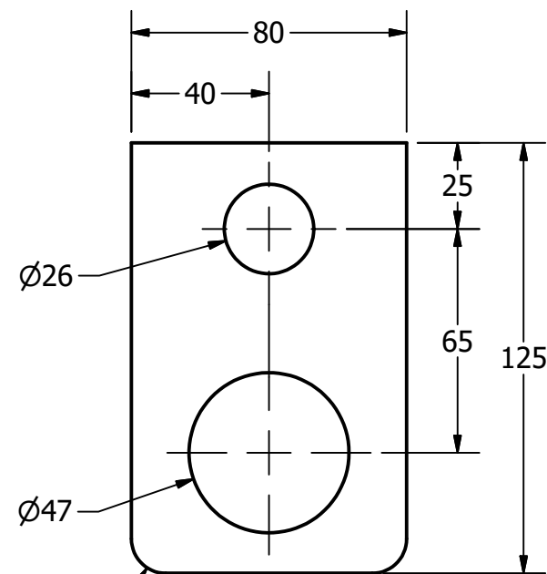
HOOK SCALE 1 / 2
