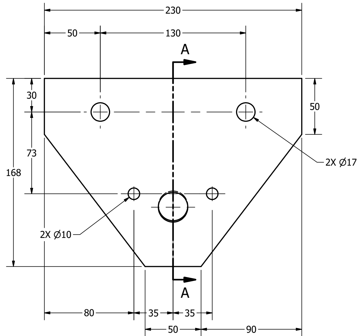
SIDE PLATE SCALE 1 / 2
