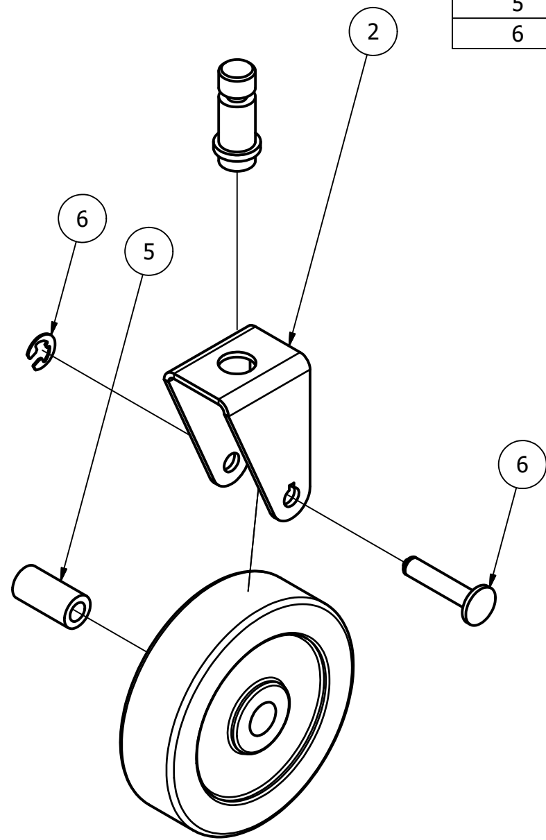
CASTER EXPLODED ASSEMBLY SCALE 1 / 2
