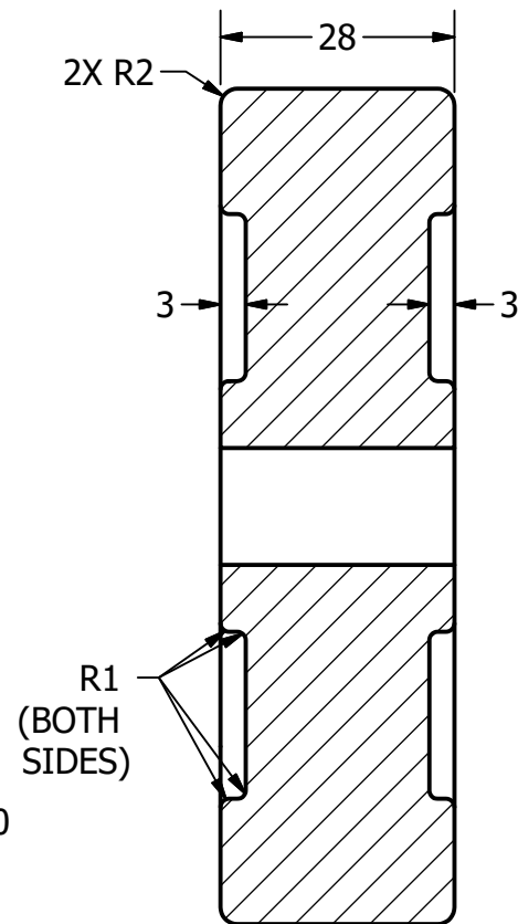
SECTION B-B SCALE 1 : 1
