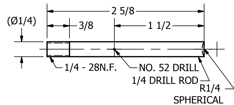
POST SCALE 1 : 1
