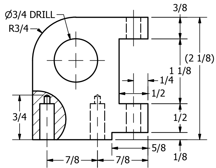
UPPER PART SCALE 1 : 1
