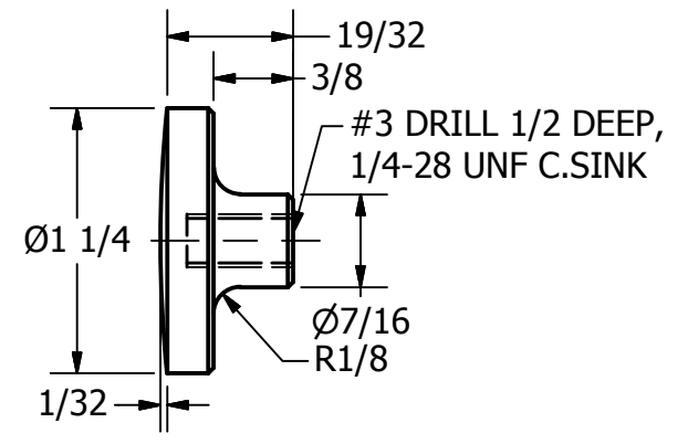
HANDLE SCALE 1 : 1
