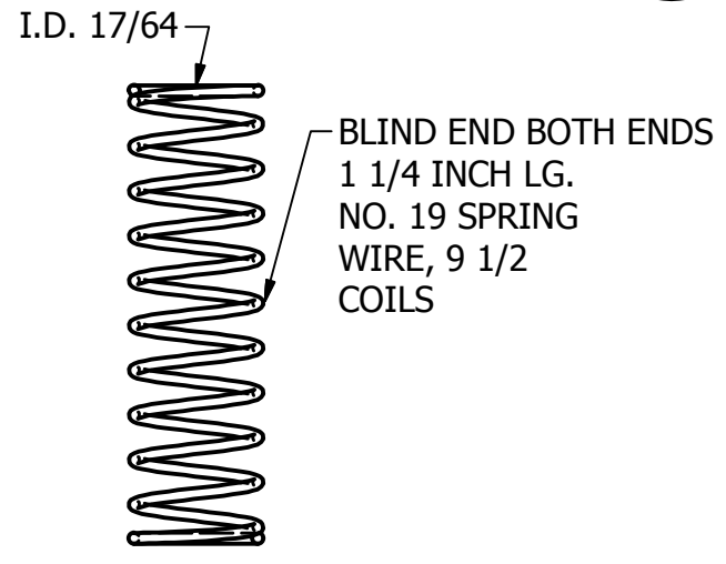
SPRING SCALE 2 : 1
