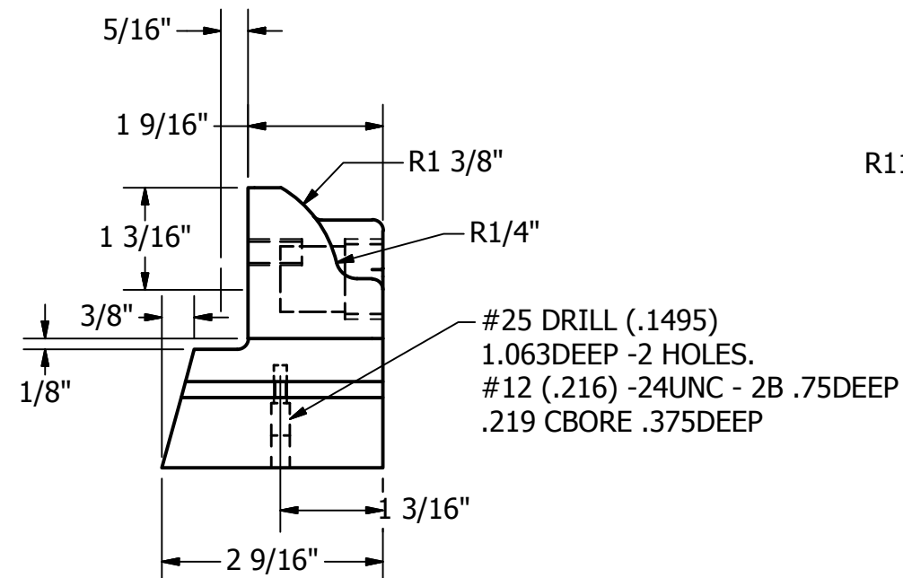
SLIDING JAW SCALE 1 / 2
