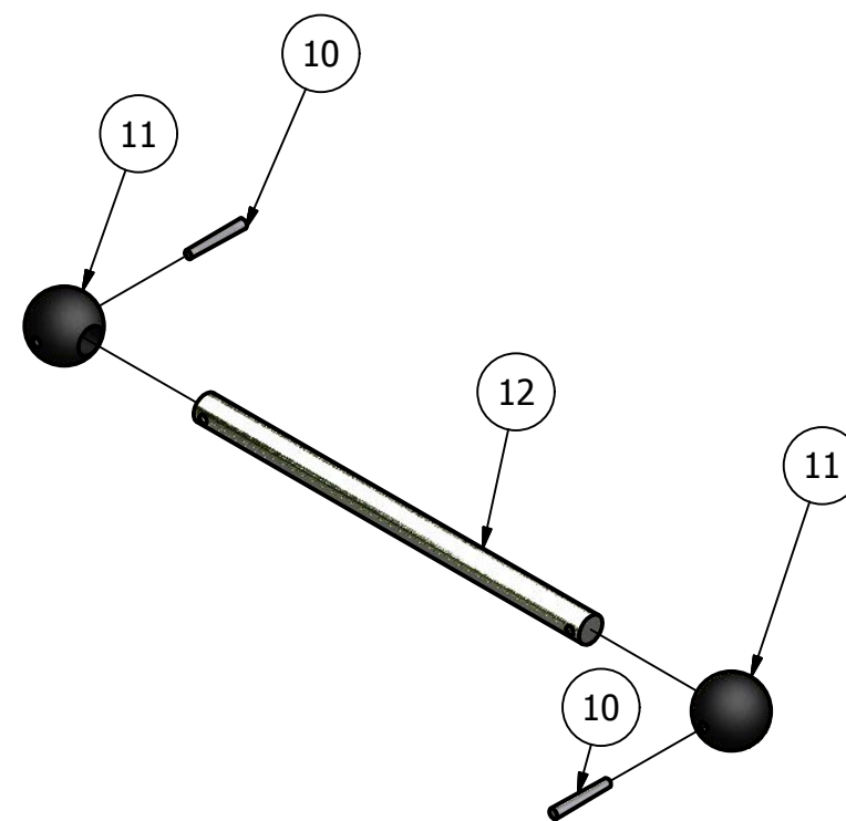
HANDEL EXPLODED SCALE 1 / 2
