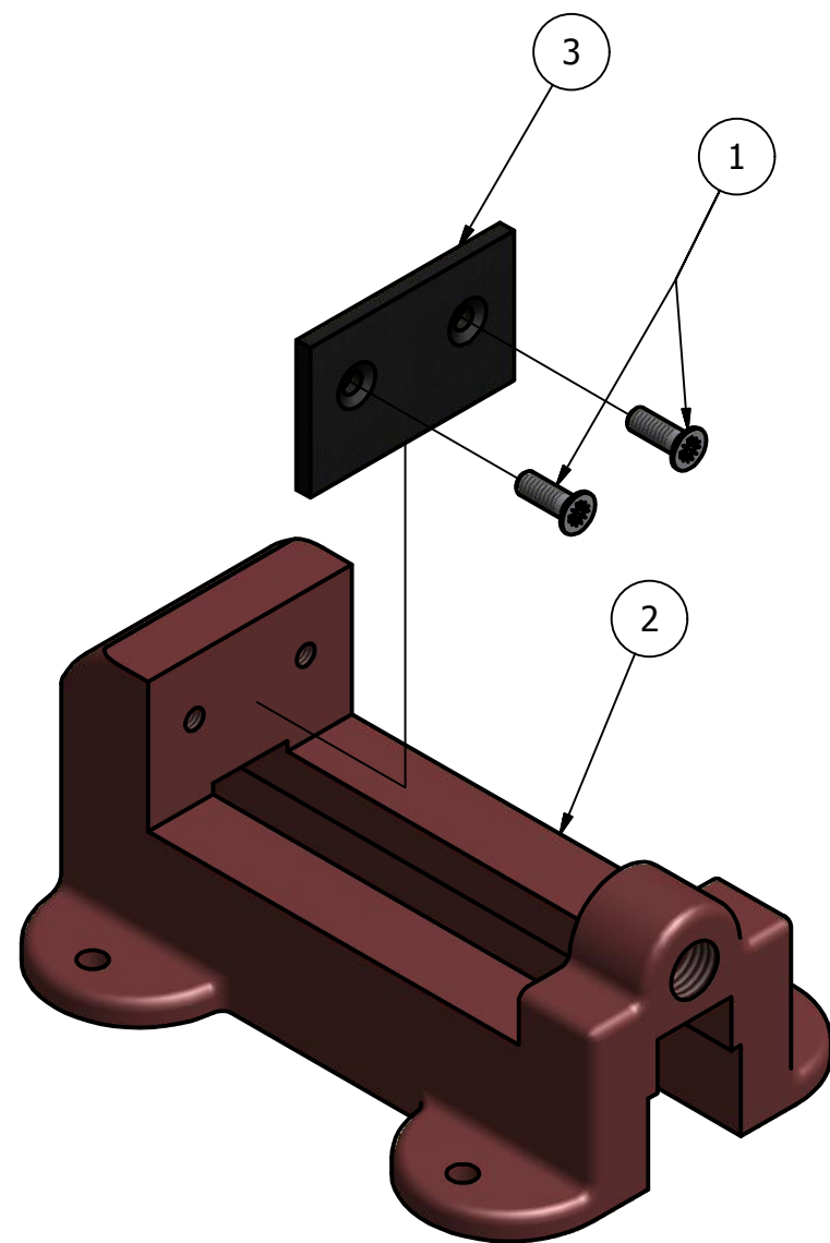
BASE EXPLODED SCALE 1 / 2
