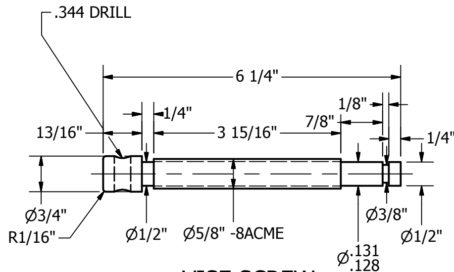
WISE SCREW SCALE 1 / 2
