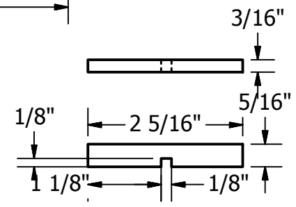
SLIDE KEY SCALE 1 / 2
