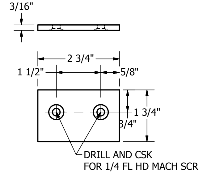
JAW PLATE SCALE 1 / 2
