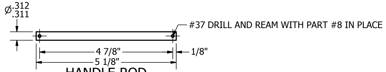
HANDLE ROD SCALE 1 / 2
