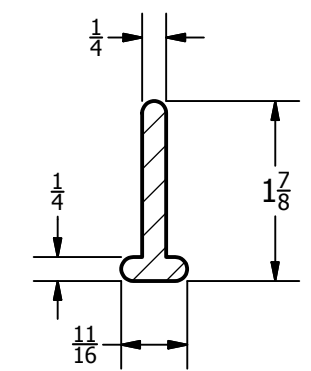
SECTION C-C SCALE 1:2
