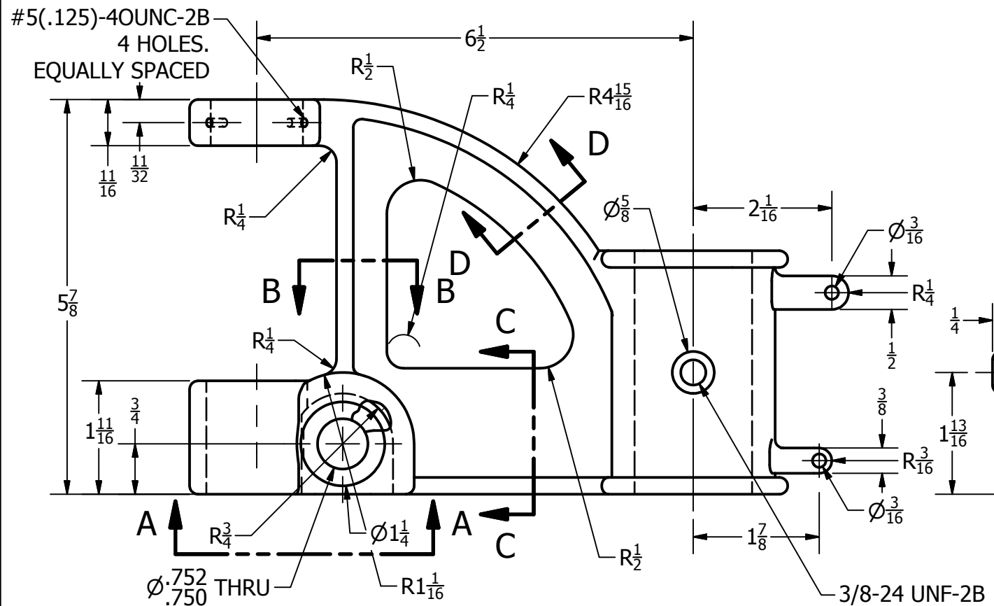
DRILL PRESS BRACKET SCALE 1:2
