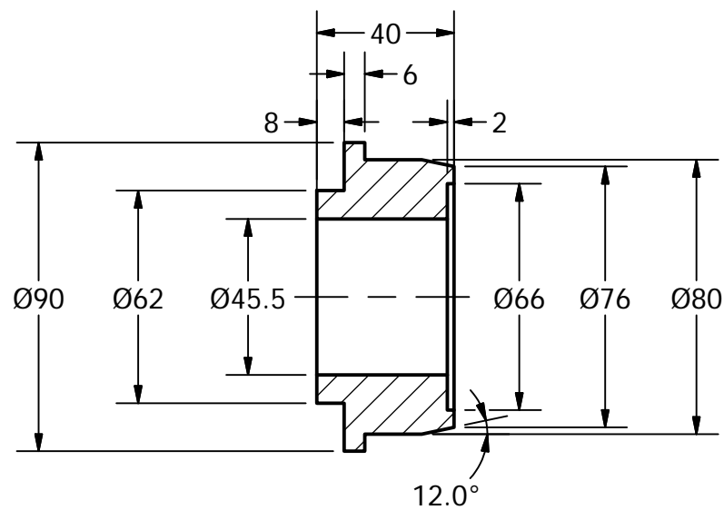
SECTION C-C SCALE 1:2
