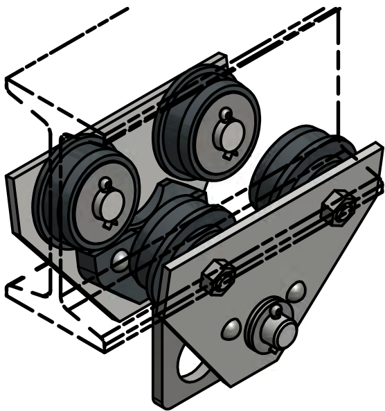
TROLLEY SCALE 1:4
