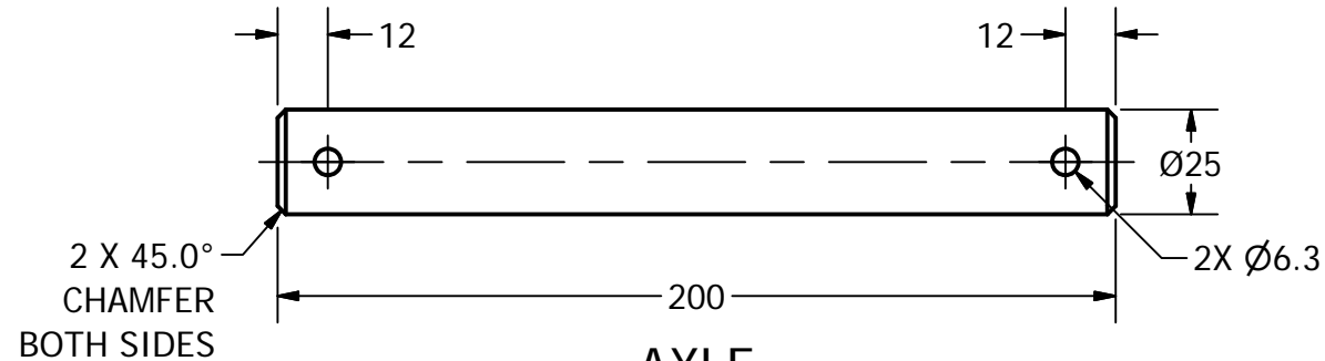
AXLE SCALE 1:2
