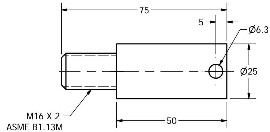
GUIDE AXLE SCALE 1:1
