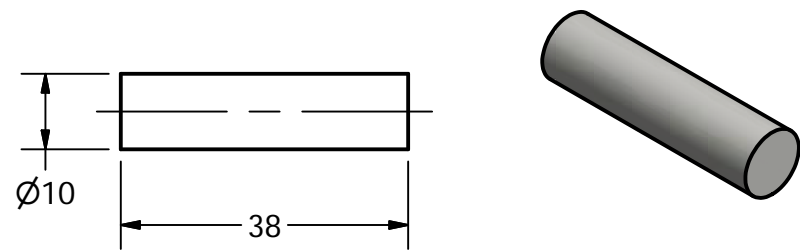
ROLLER BEARING SCALE 1:1
