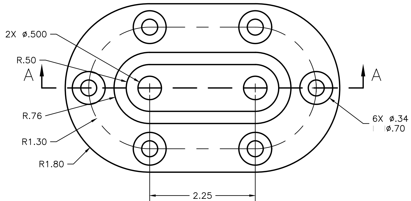
SHAFT BASE SCALE 1:1
