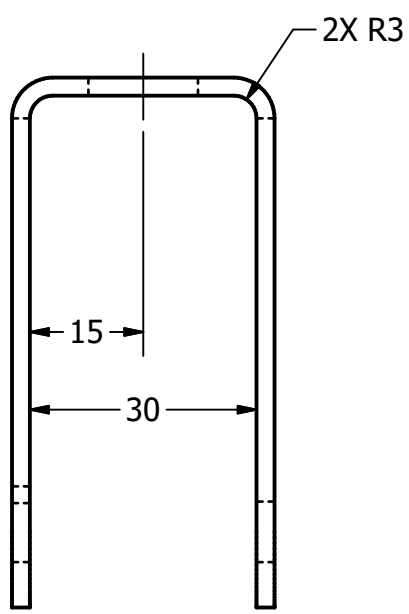
BRACKET FOLDED SCALE 1 : 1
