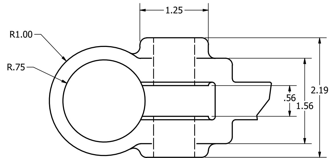
VIEW A-A SCALE 1 / 1
