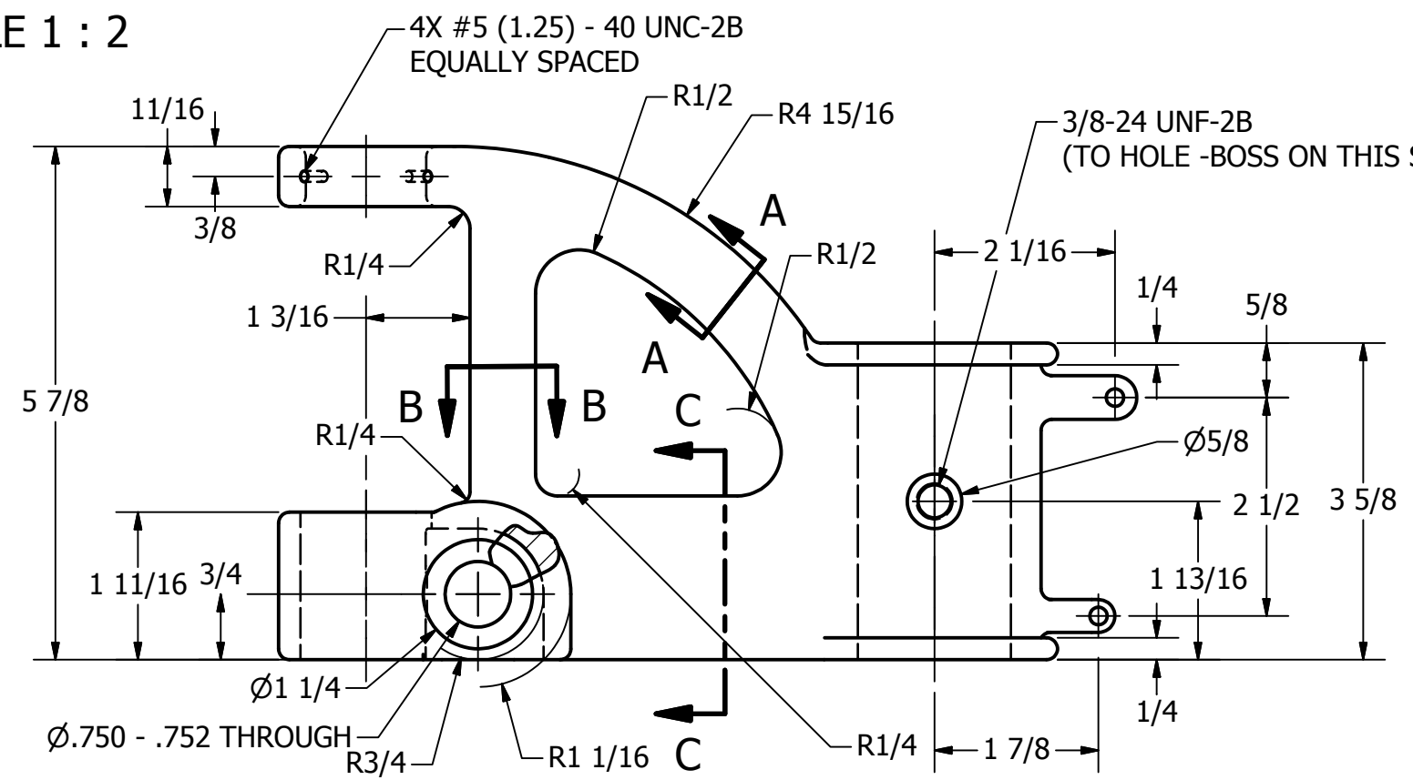
VIEW D-D SCALE 1 : 2
