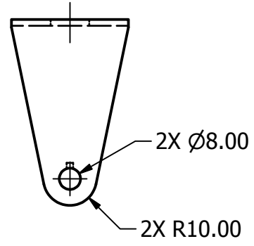
BRACKET SCALE 1 : 1
