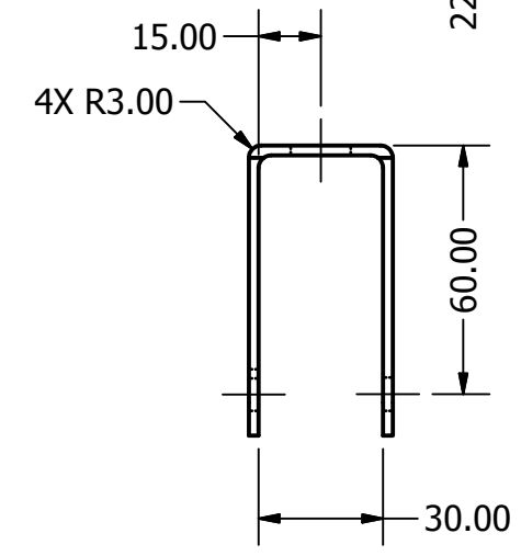
BRACKET SCALE 1 / 2
