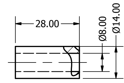
BUSHING SCALE 1 : 1
