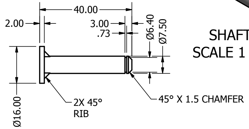
SHAFT SCALE 1 : 1
