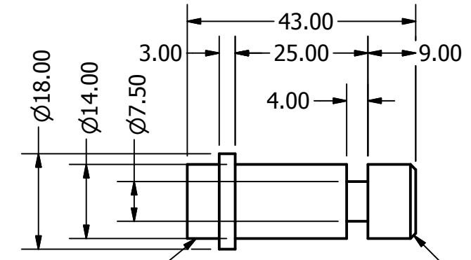
POST SCALE 1 : 1
