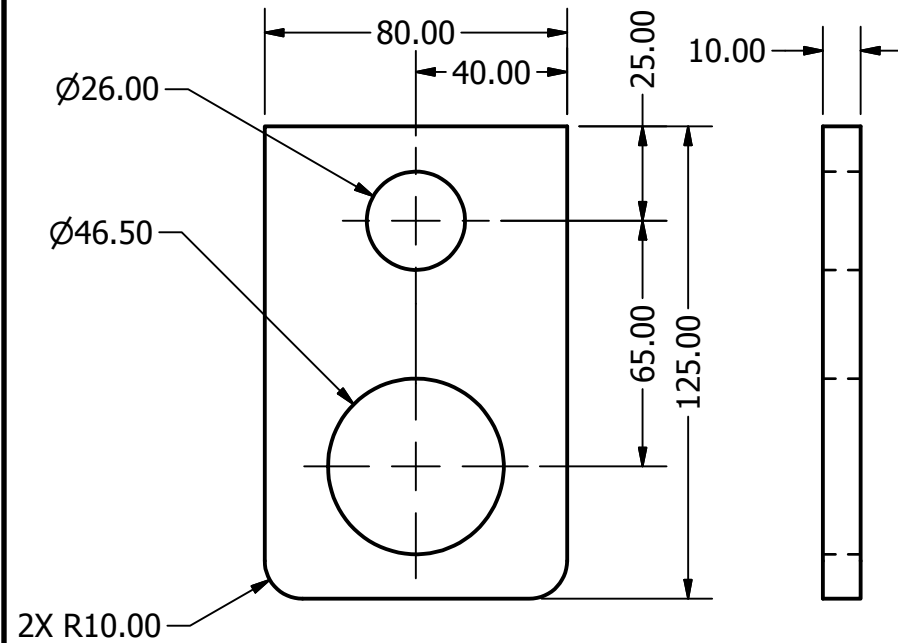
HOOK SCALE 1/2
