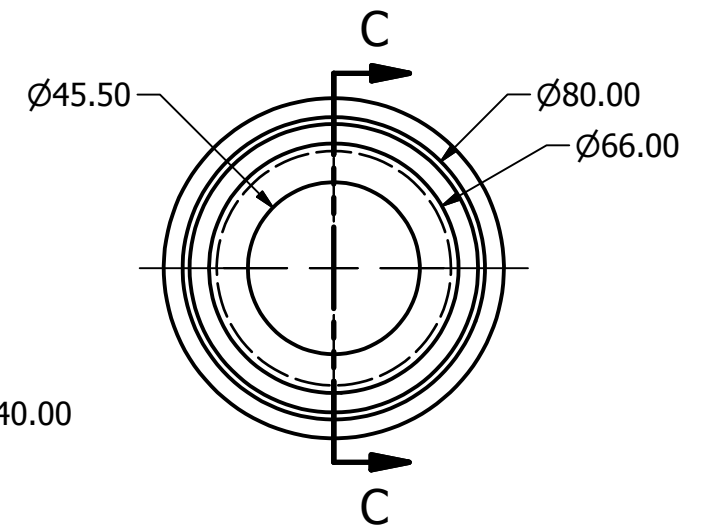
WHEEL SCALE 1/2
