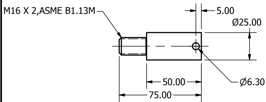
AXLE SCALE 1/2
