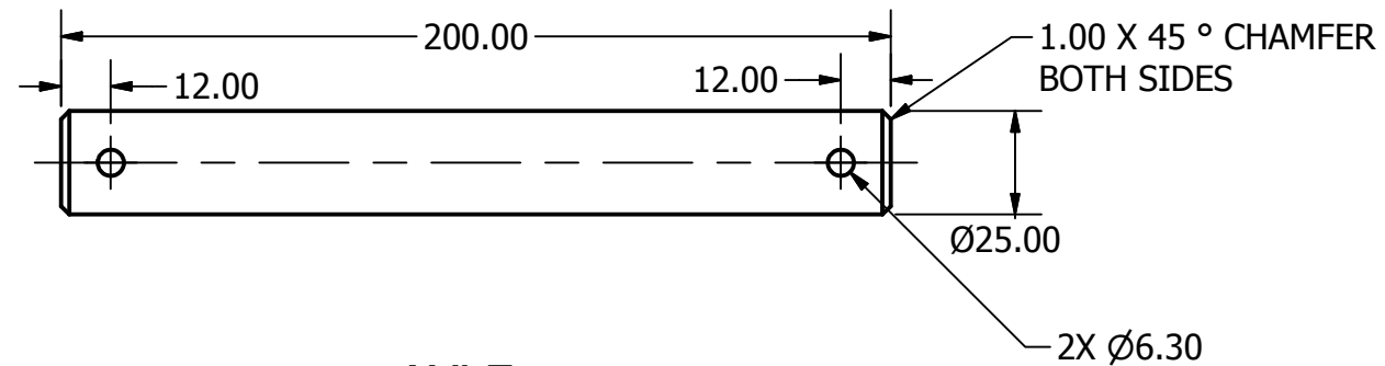
AXLE SCALE 1/2
