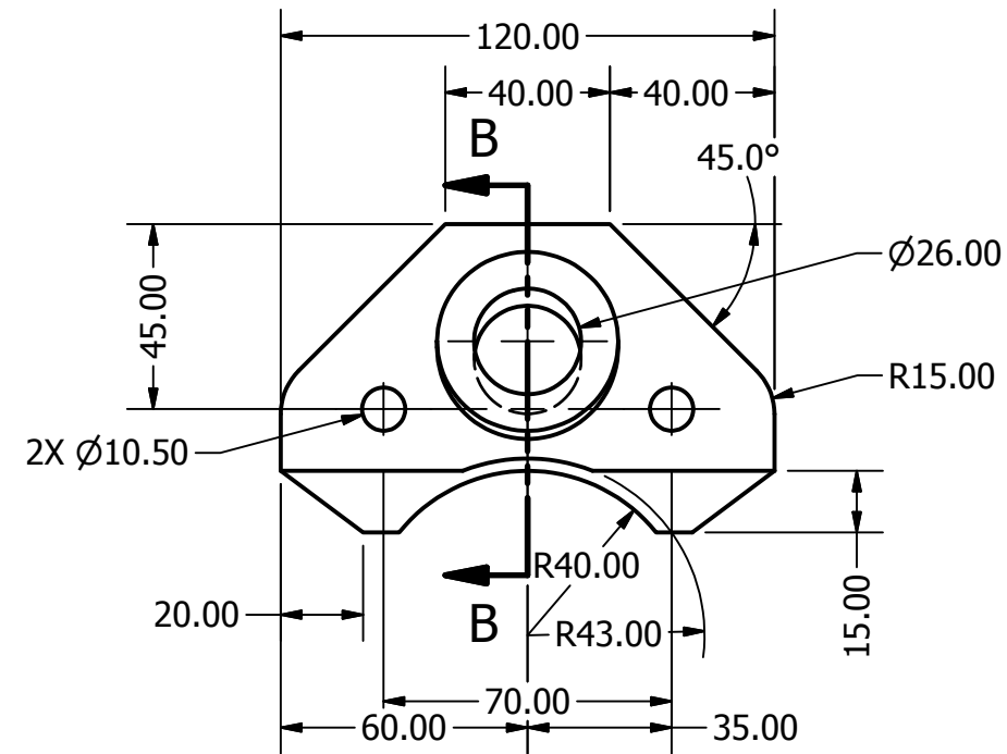
GUIDE SCALE 1/2
