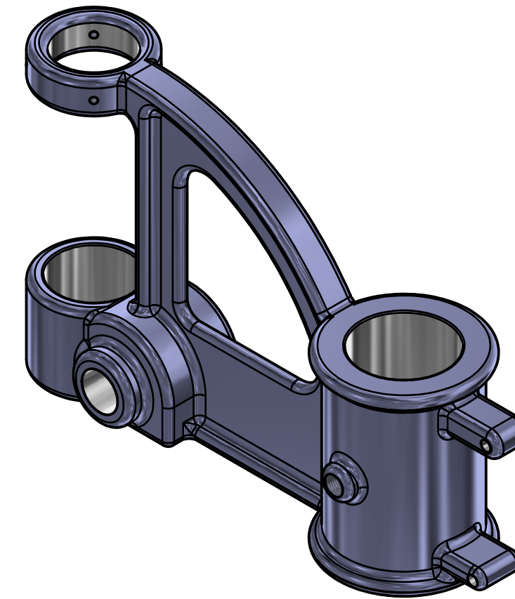
ISOMETRIC SCALE 1:2
