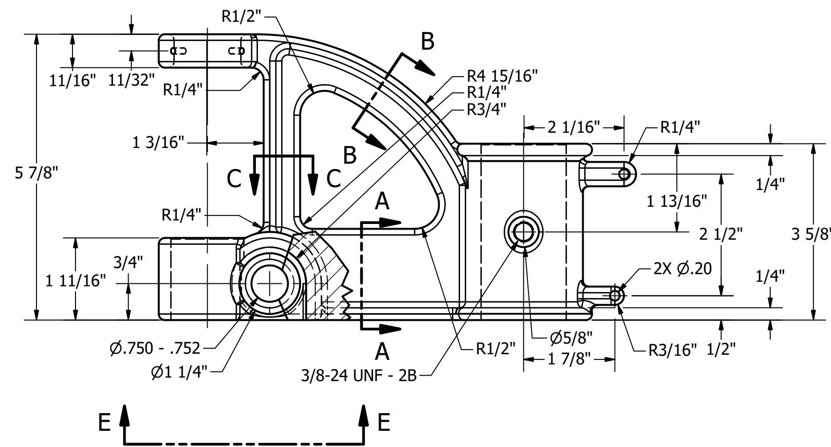
DRILL PRESS BRACKET SCALE 1:2
