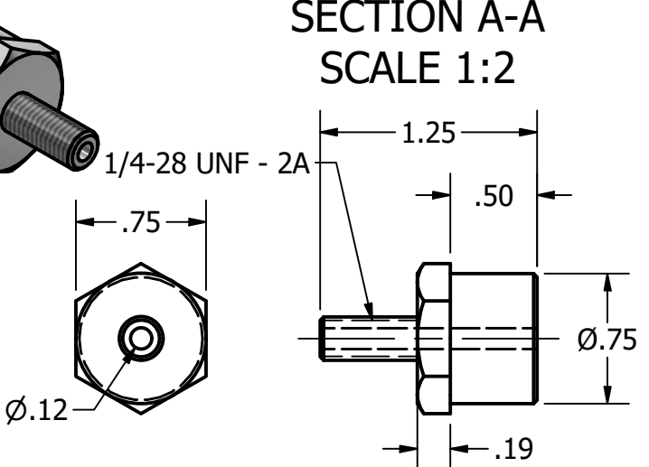
VACUUM CONNECTOR SCALE 1:1
