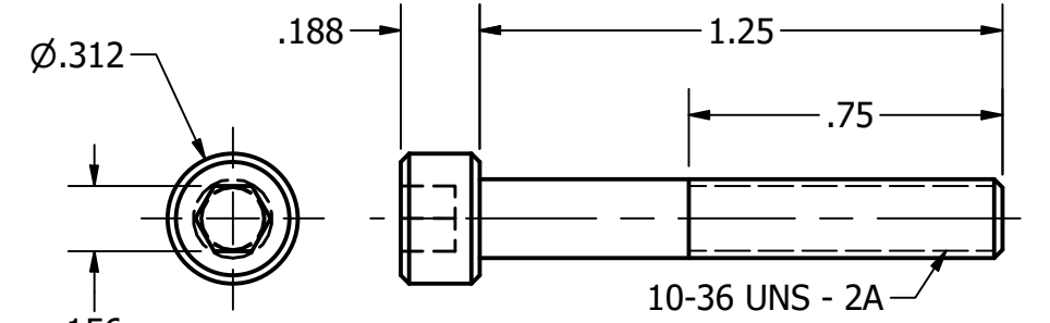
CAP SCREW SCALE 2:1
