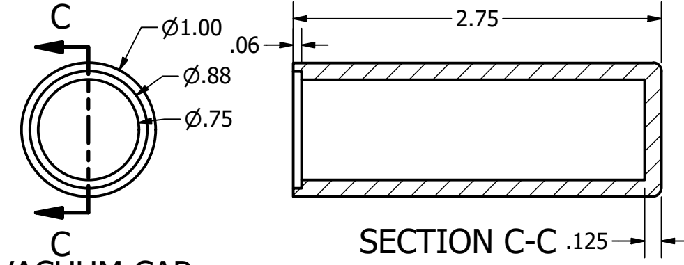
C VACUUM CAP SCALE 1:1
