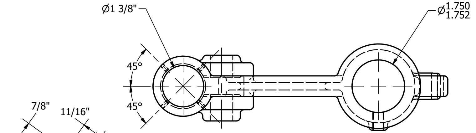
TOP VIEW SCALE 1 / 2
