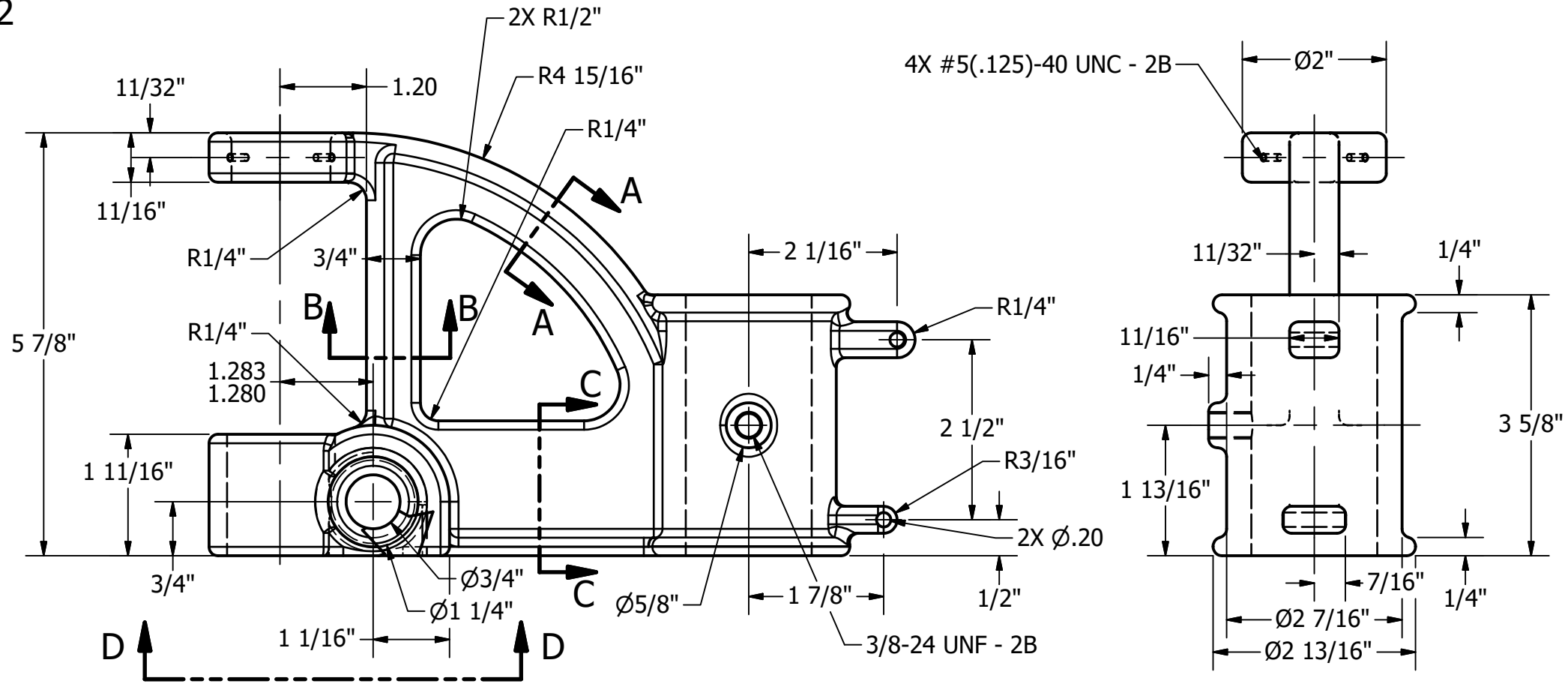
RIGHT VIEW SCALE 1 / 2
