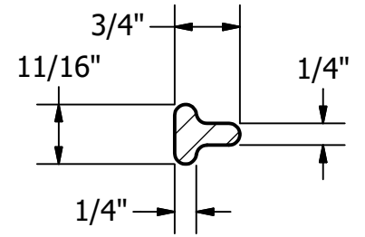
SECTION B-B SCALE 1 / 2
