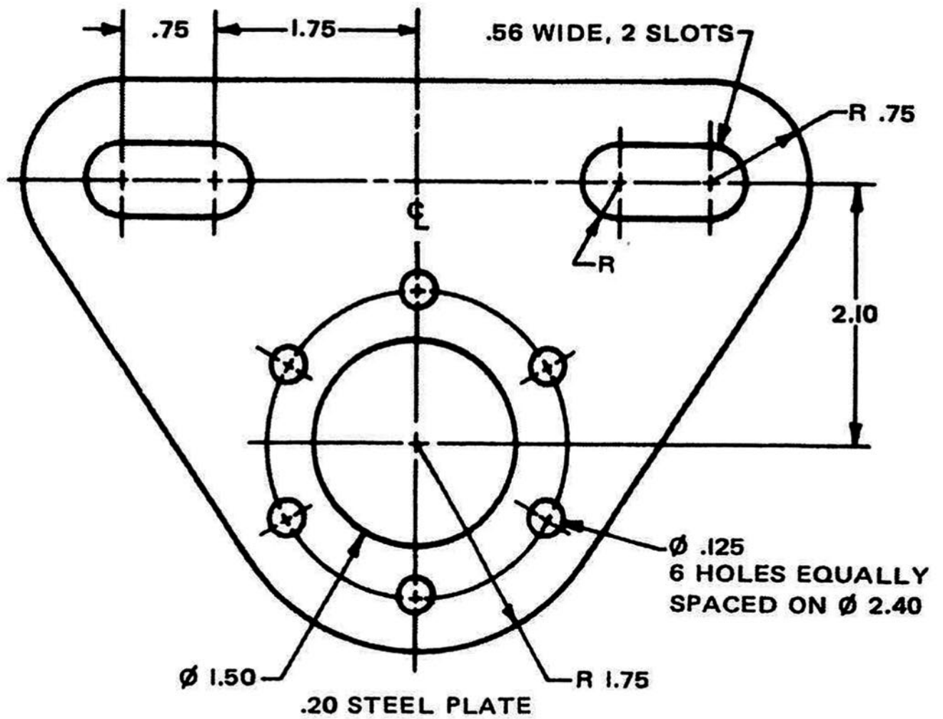
Fig. 4-39 Shaft support.
