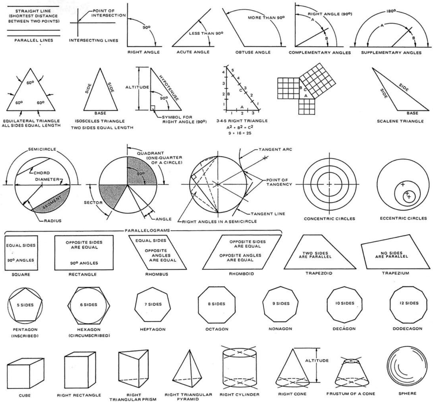
Fig. 5-1 Dictionary of drafting geometry.
