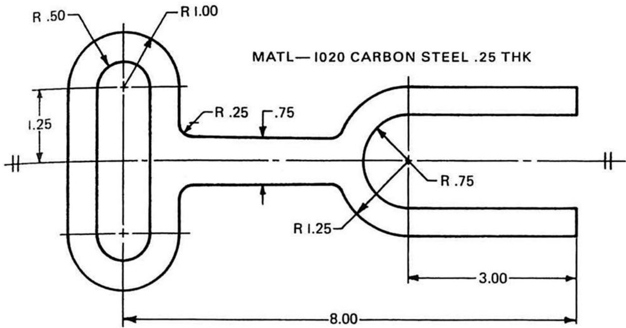
Fig. 5-31 Adjustable fork.
