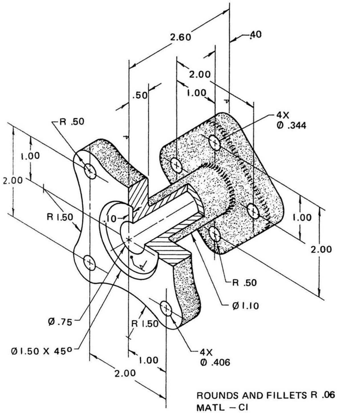
Fig. 6-111 Flanged adaptor.
