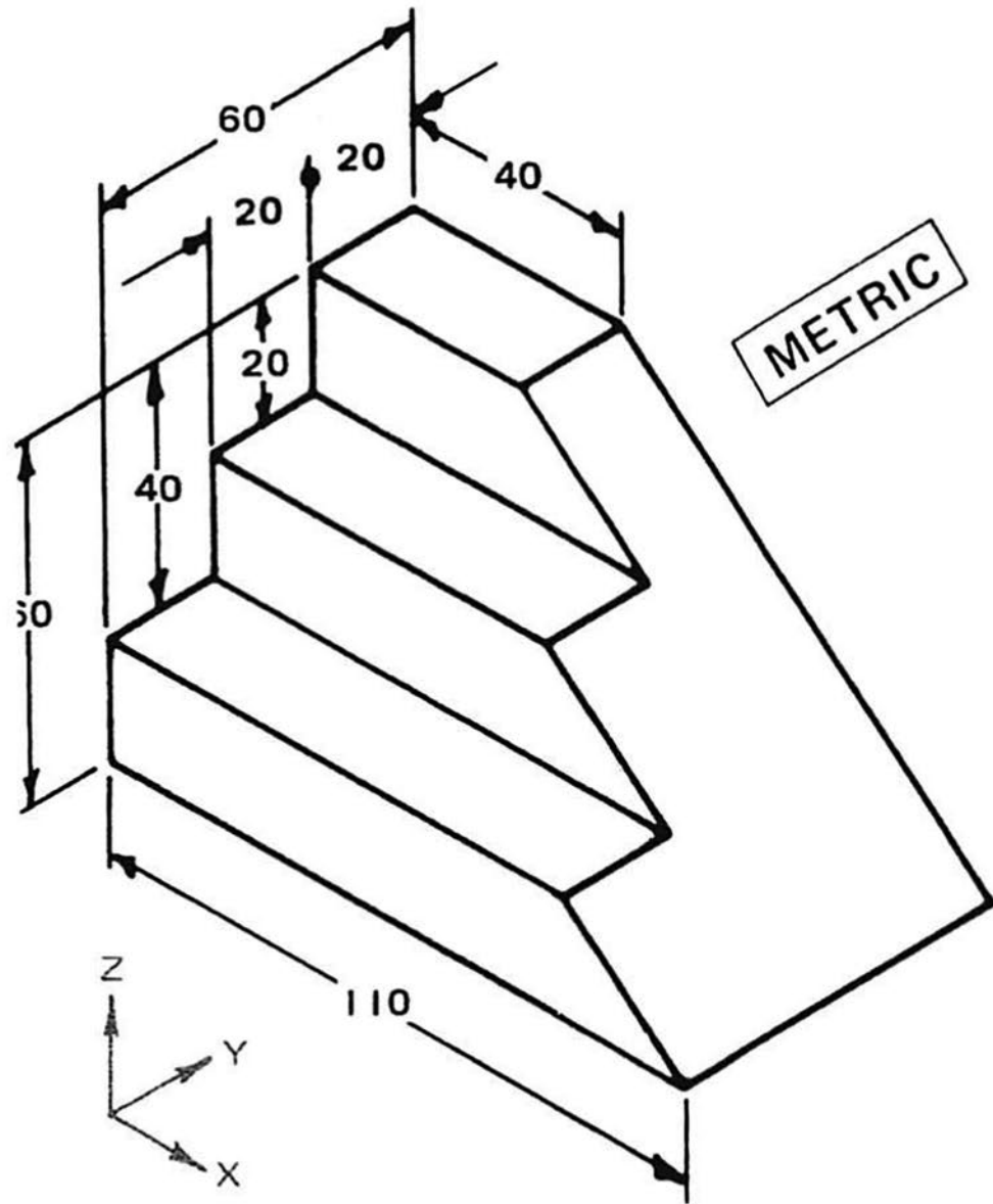
Fig. 6-80 Adjusting guide.
