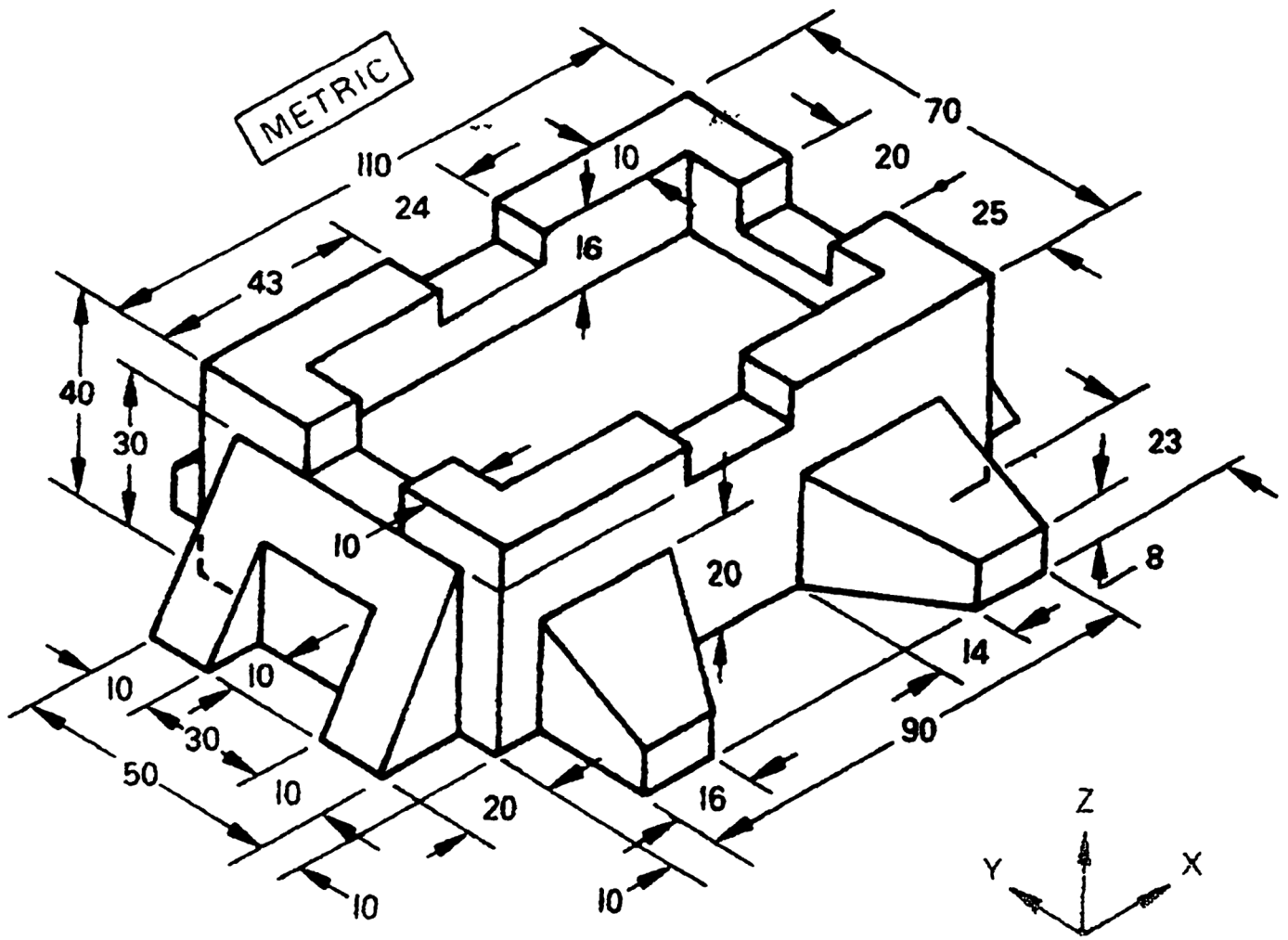
Fig. 6-86 Base plate.
