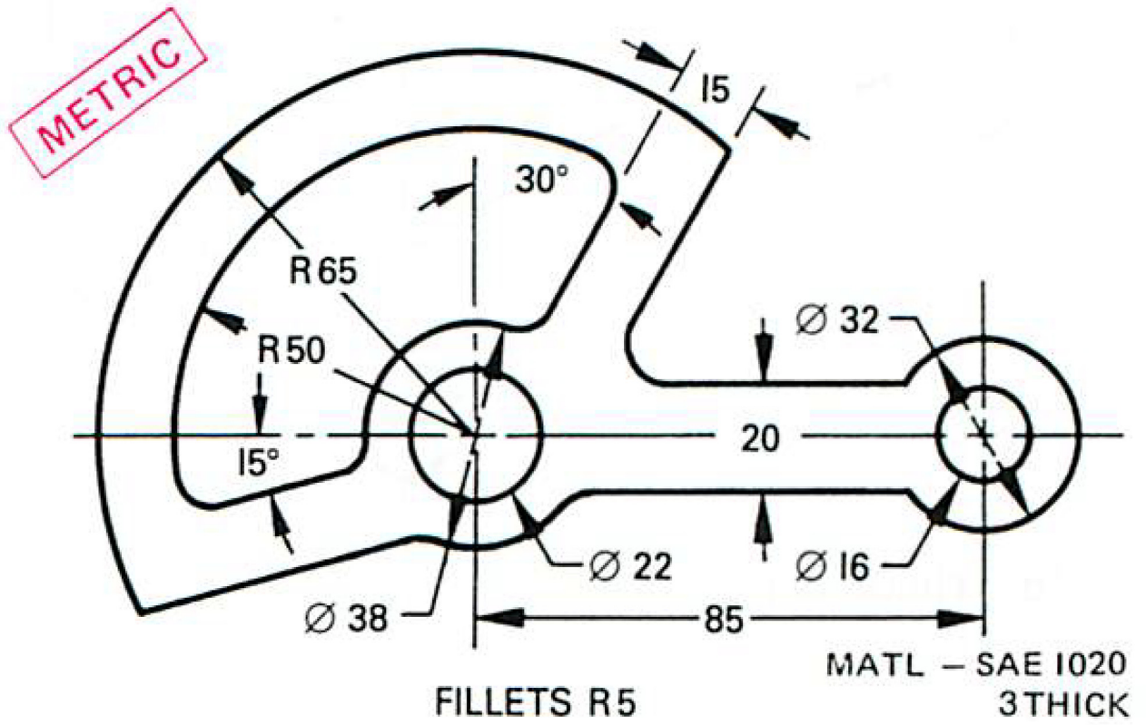
Fig. 8-86 Adjustable sector.
