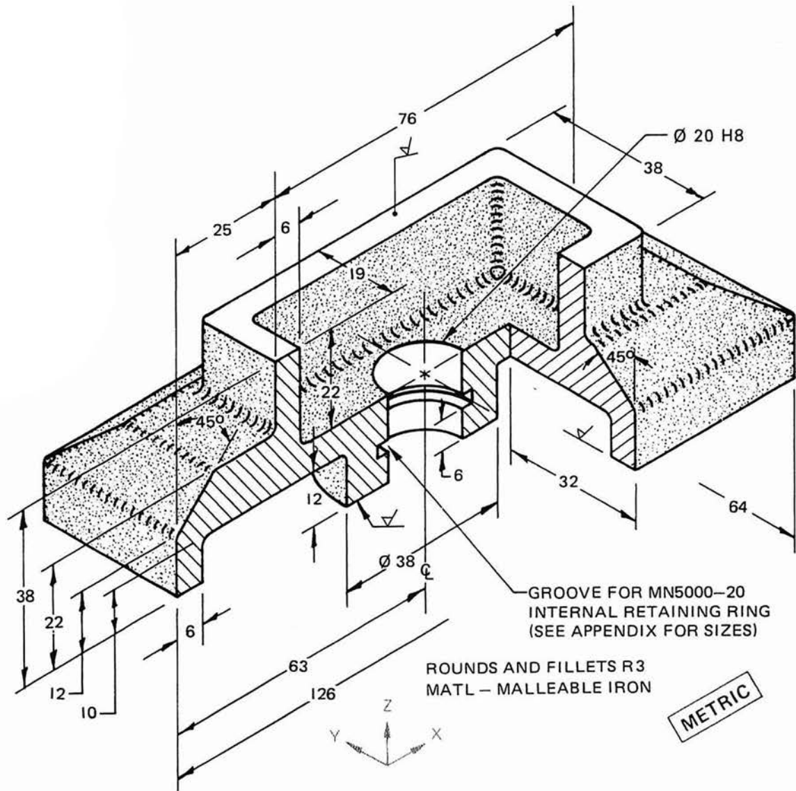
Fig. 9-68 Hold-down bracket.
