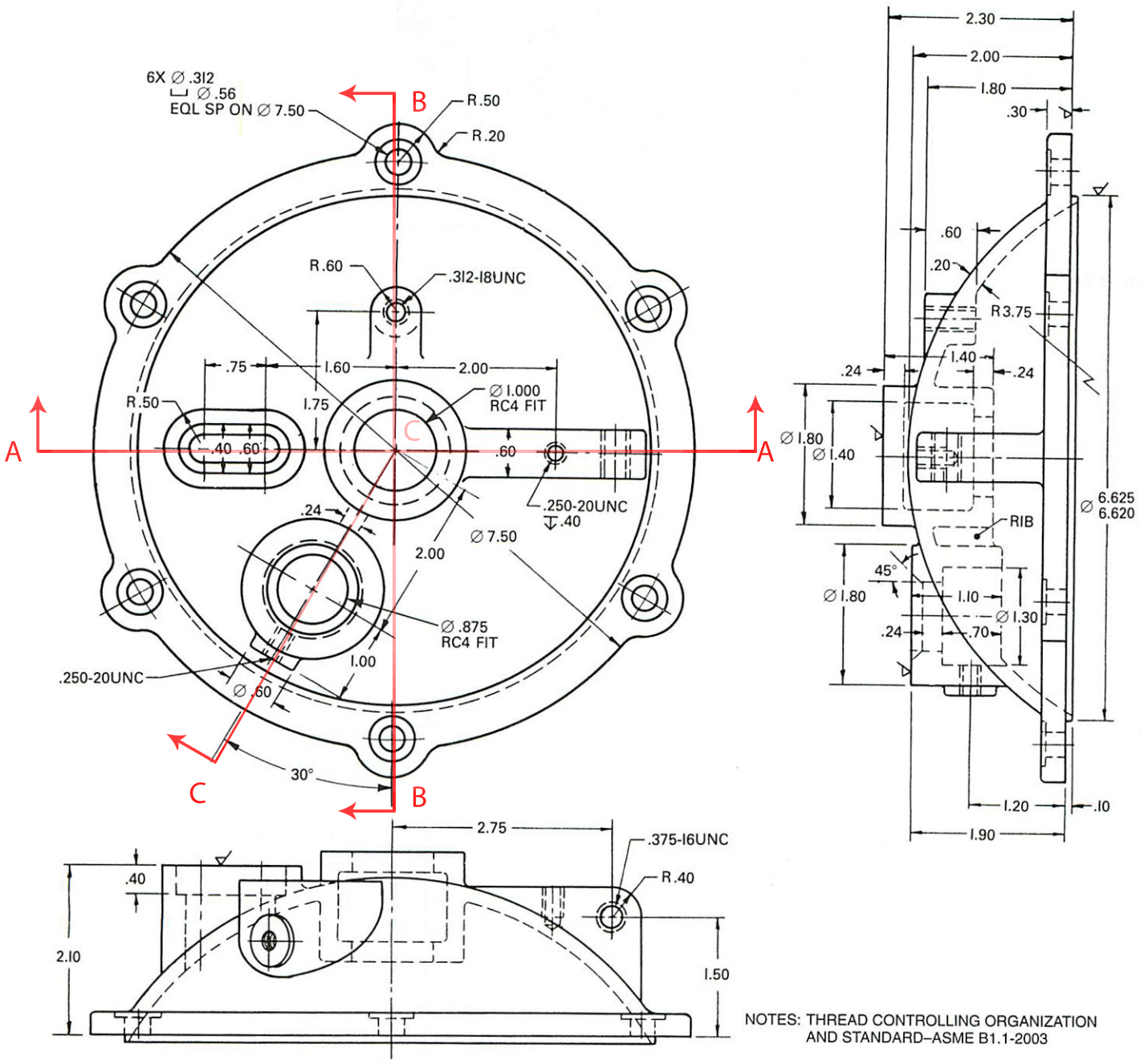
Fig. 9-72 Domed cover.
