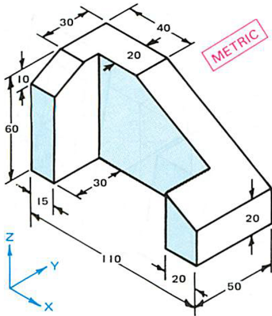
Fig. 6-81 Flanged support.
