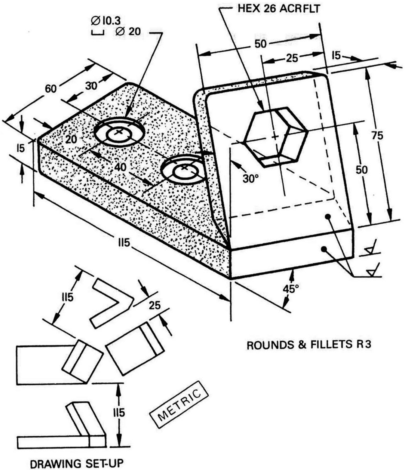
Fig. 7-58 Hexagon slot support.
