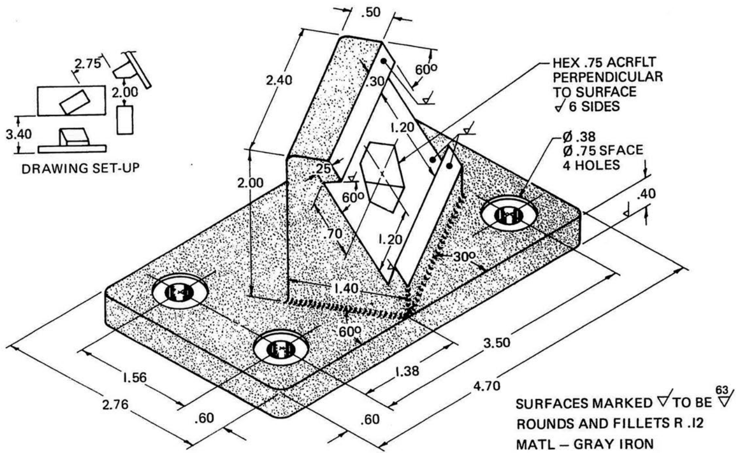
Fig. 7-59 Dovetail bracket.
