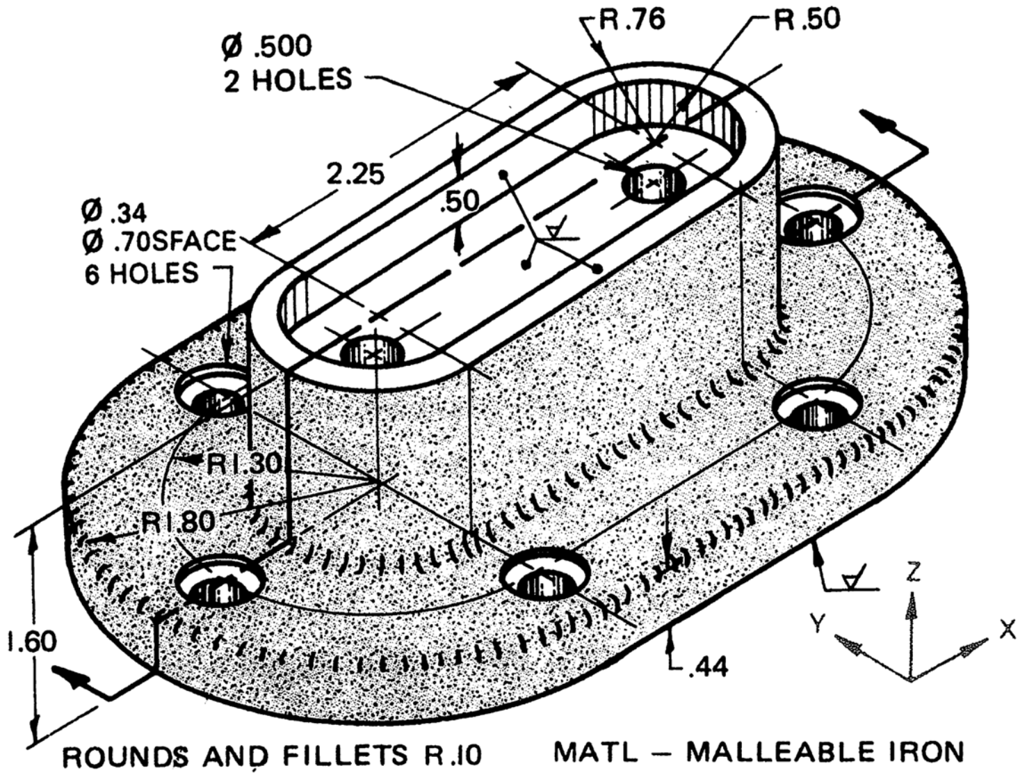
Fig. 9-35 Shaft base.
