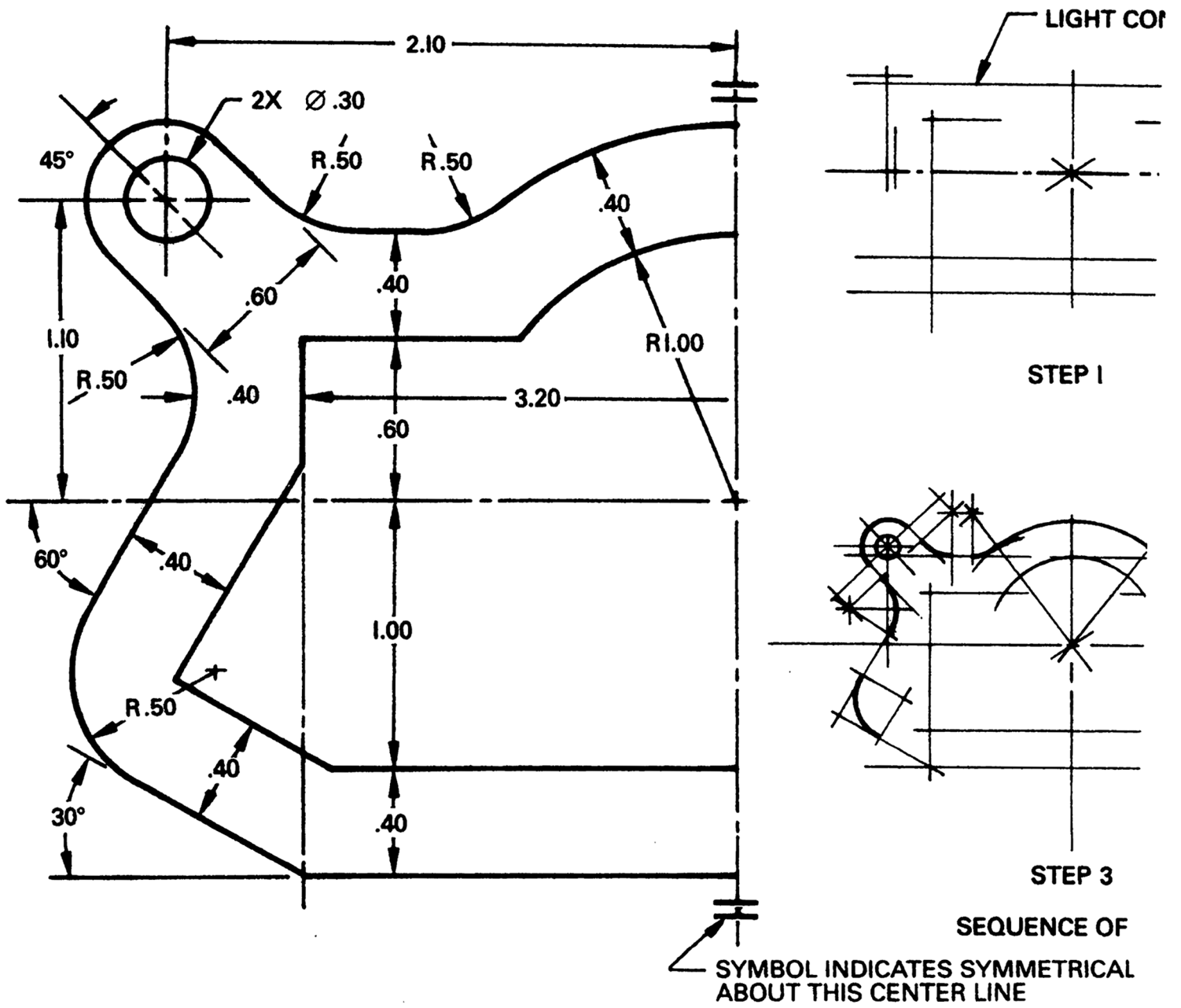
Fig. 4-36 Gasket.
