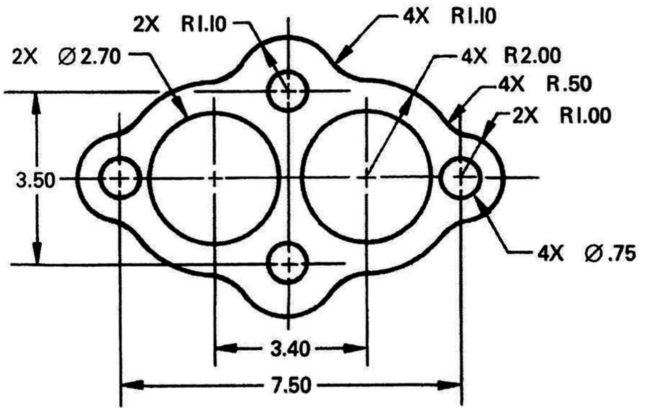
Fig. 4-38 Carburetor gasket.
