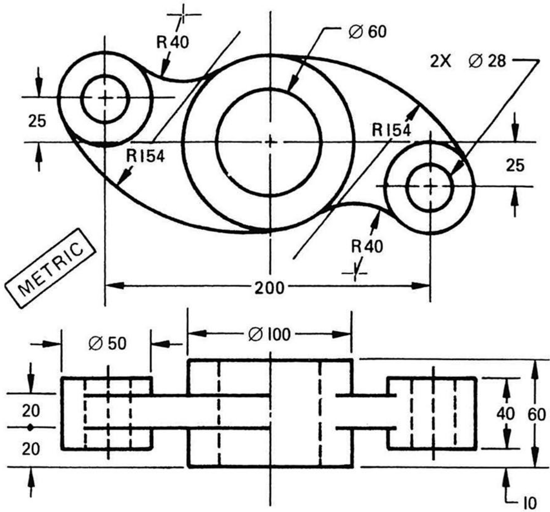
Fig. 5-32 Rocker arm.
