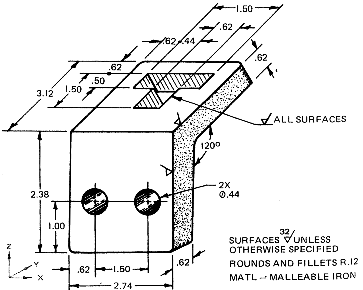
Fig. 7-43 Angle bracket.
