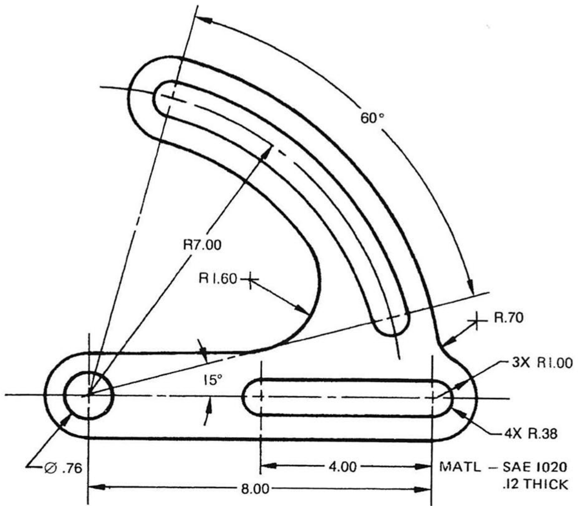
Fig. 8-83 Adjustable table support.
