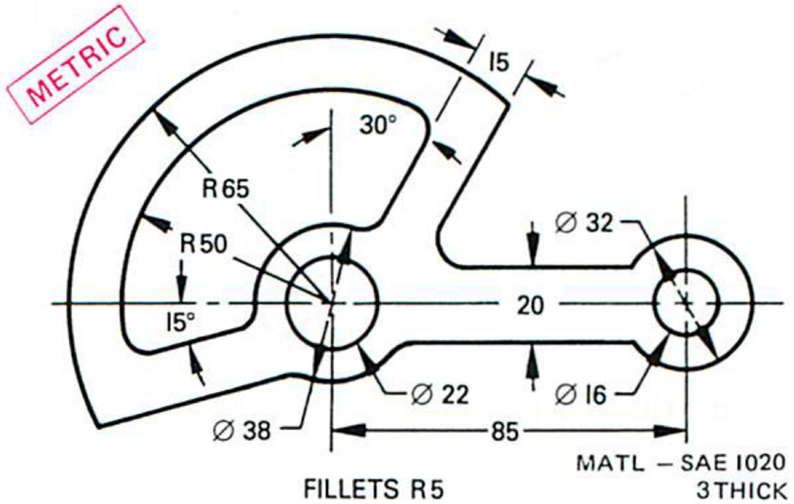
Fig. 8-86 Adjustable sector.
