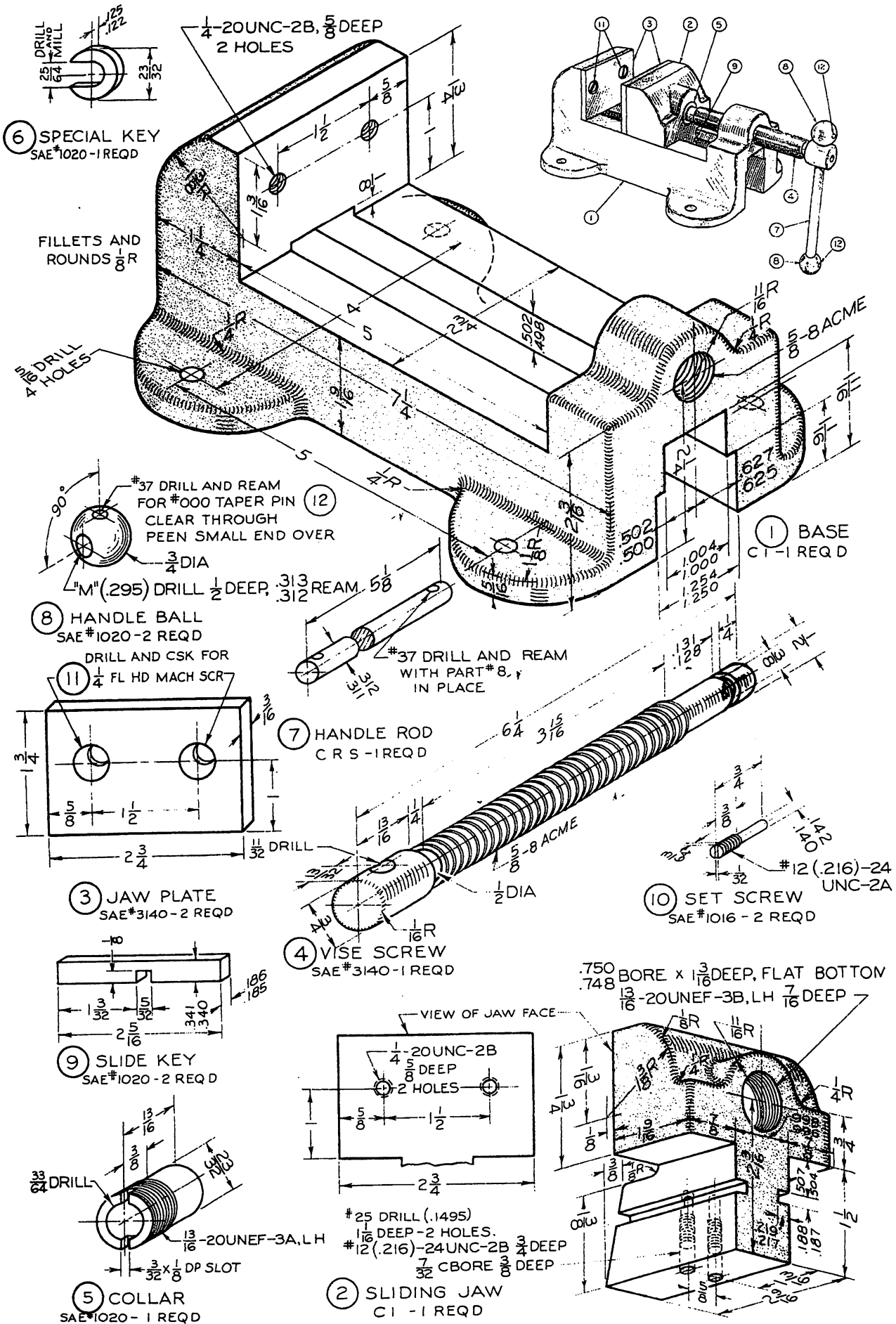
Fig. 14-71 Machine Vise. (1) Draw details. (2) Draw assembly. If assigned, convert dimensions to the decimal system
