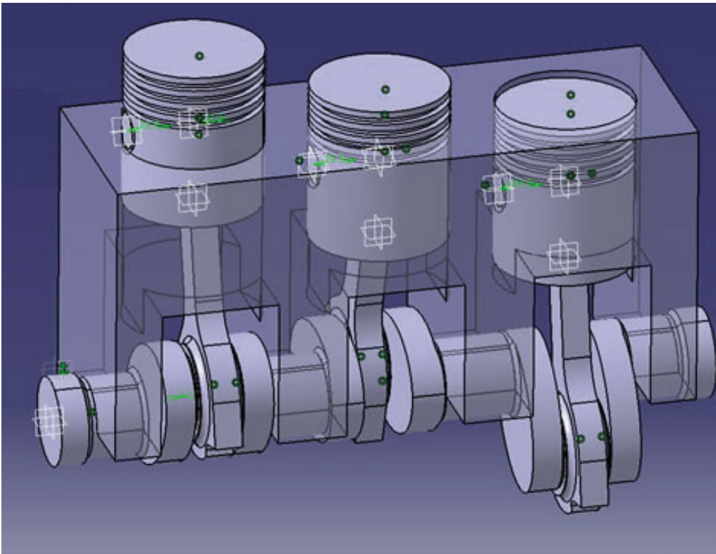
Operational Test Assembly Model: Working Crankshaft and Pistons in Engine Block
