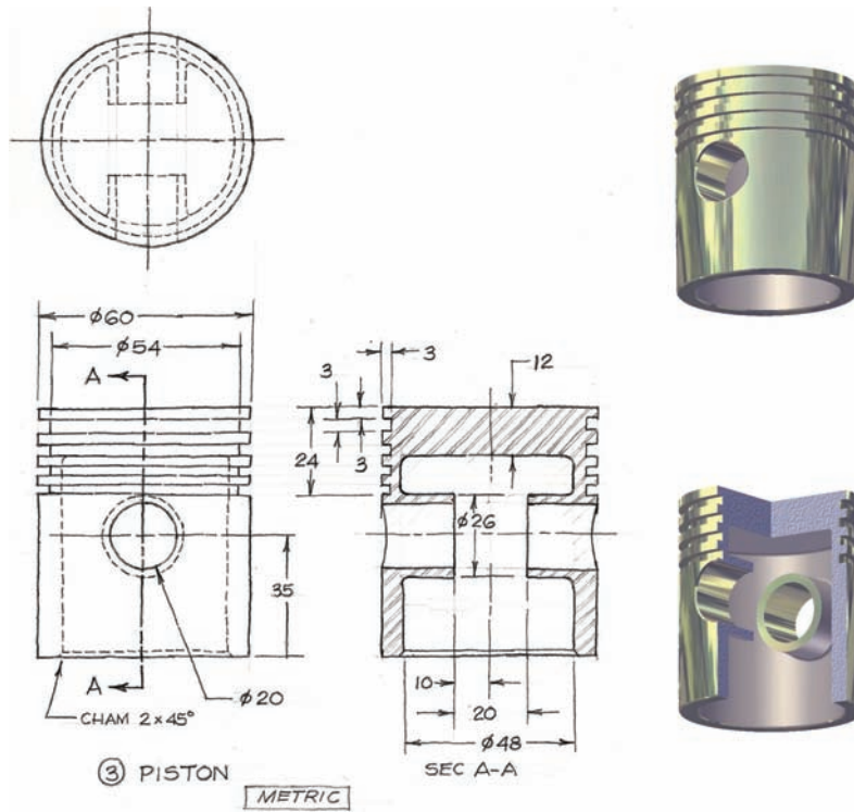
Sketch for Part Number 3: PISTON
