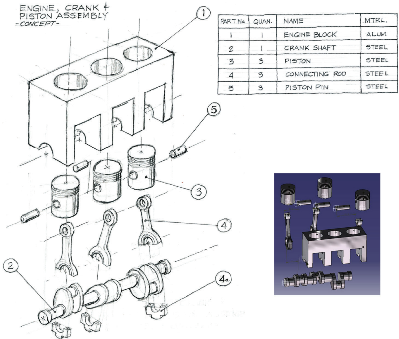
Concept Sketch and Parts for Virtual Engine Assembly
