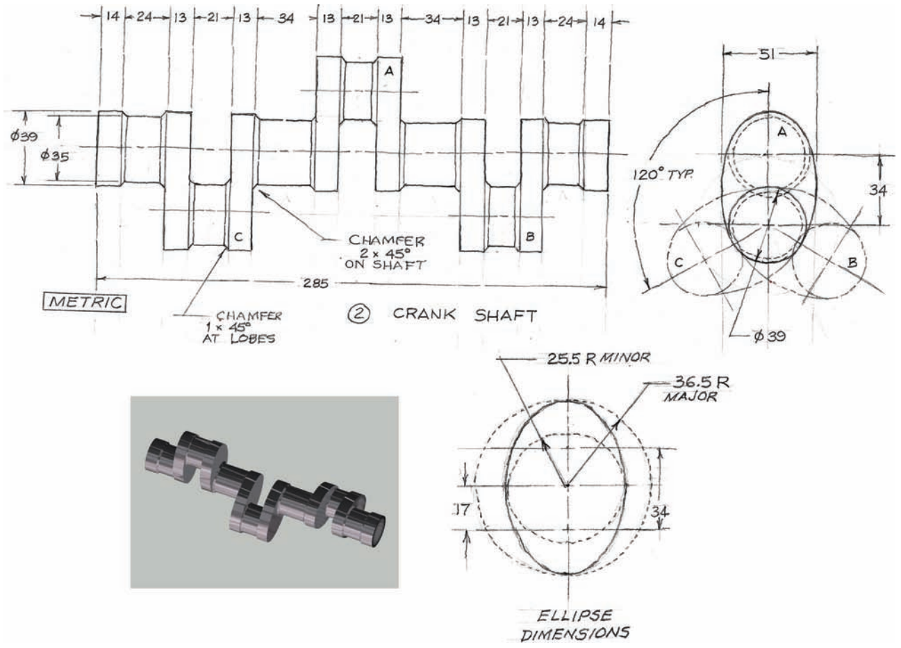
Sketch for Part Number 2: CRANK SHAFT
