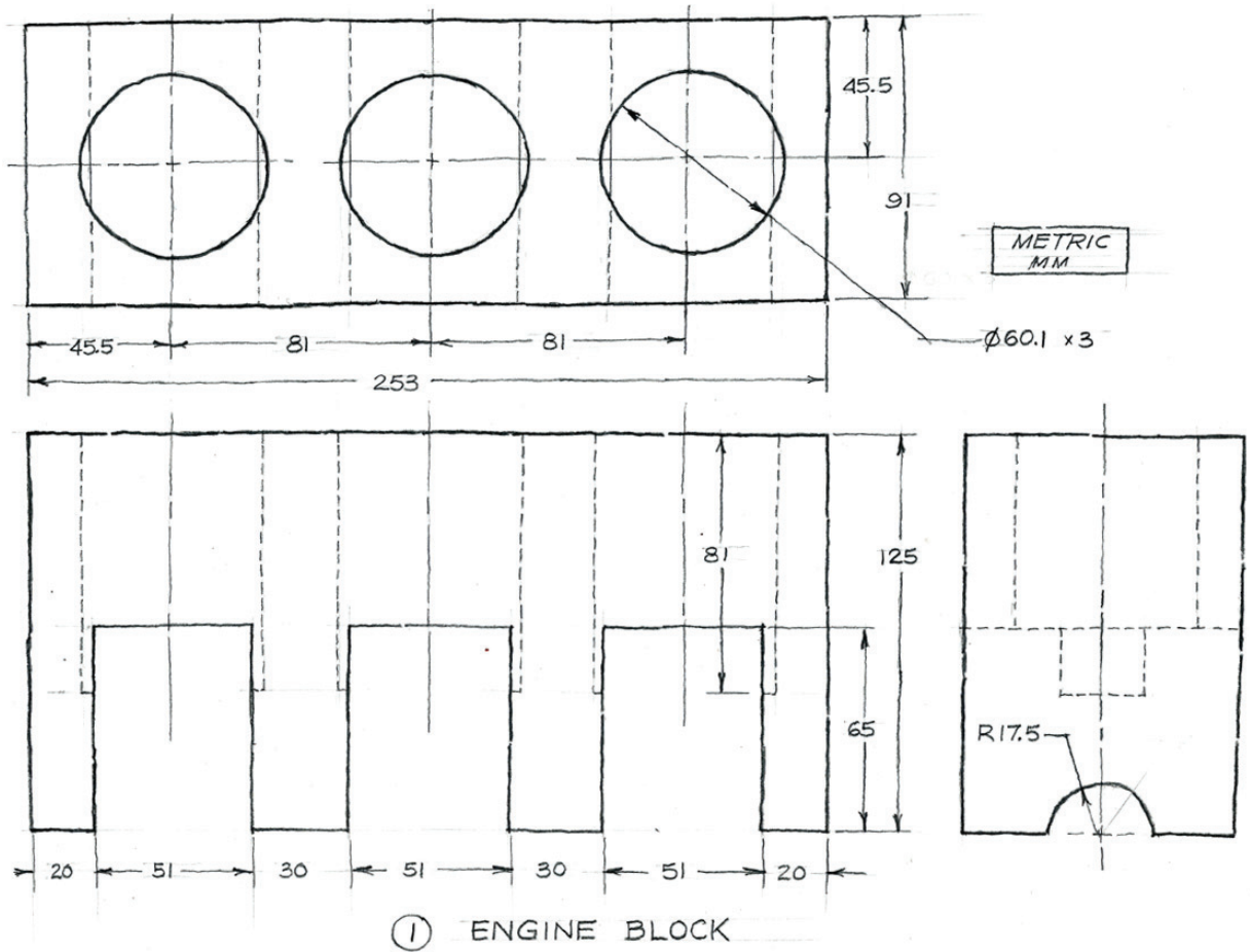
Sketch for Part Number 1: ENGINE BLOCK
