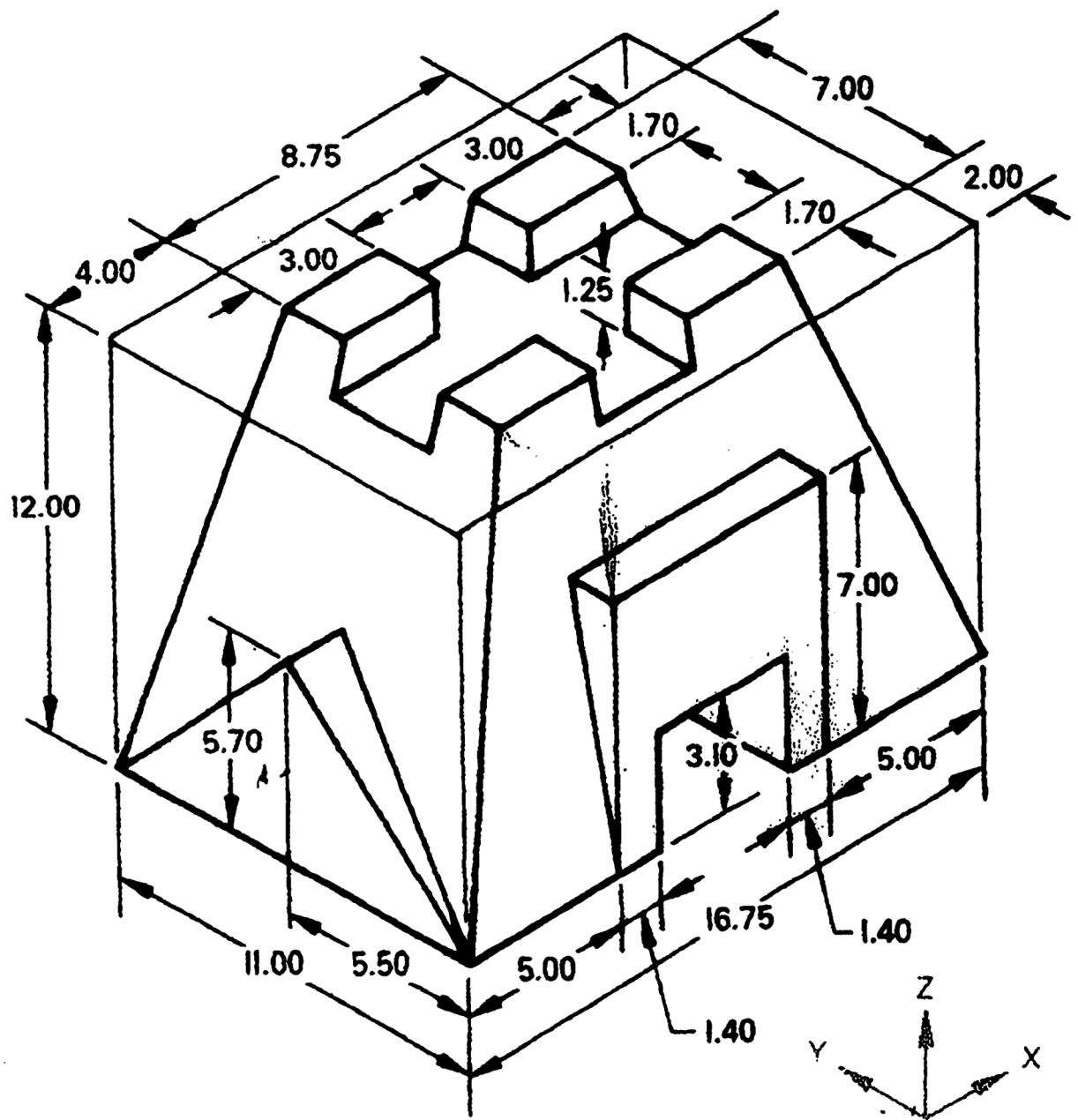
Fig. 6-85 Angle block (symmetrical).
