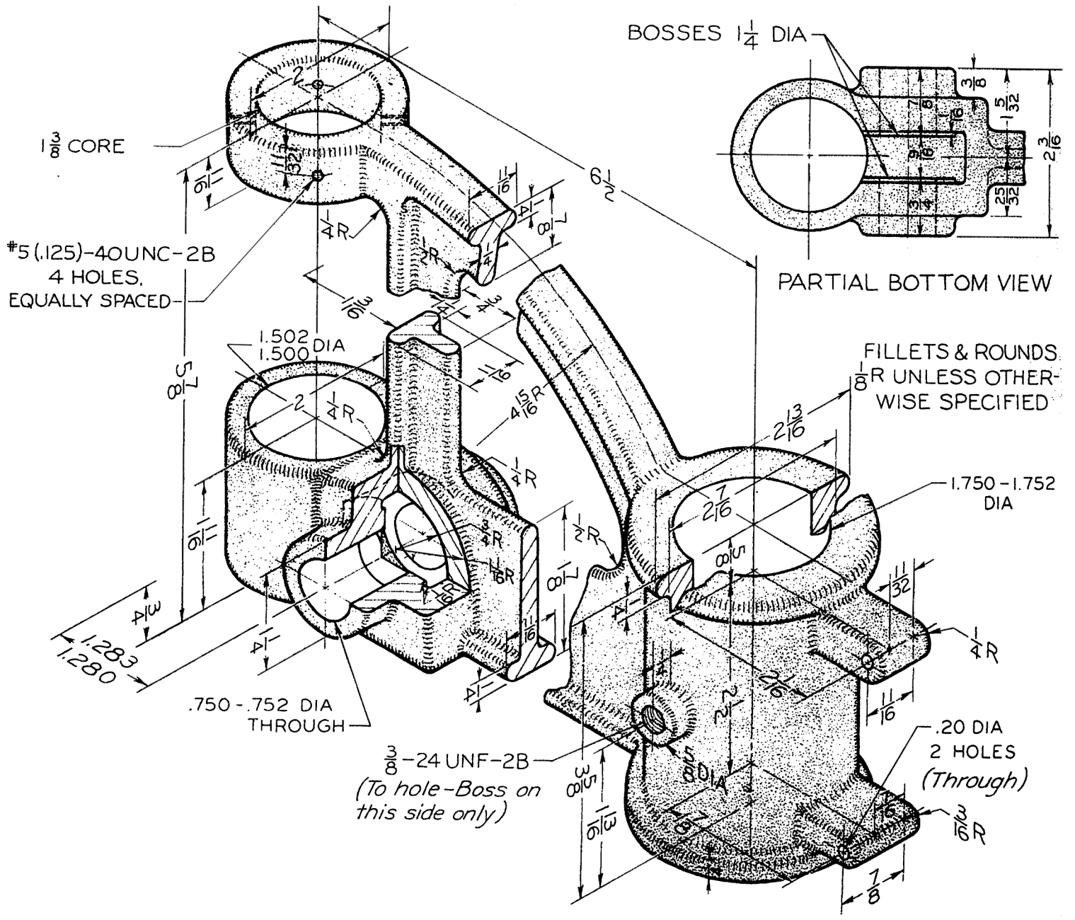
Fig. 14-35 Drill Press Bracket. Make detail drawing. Use Size C sheet.
