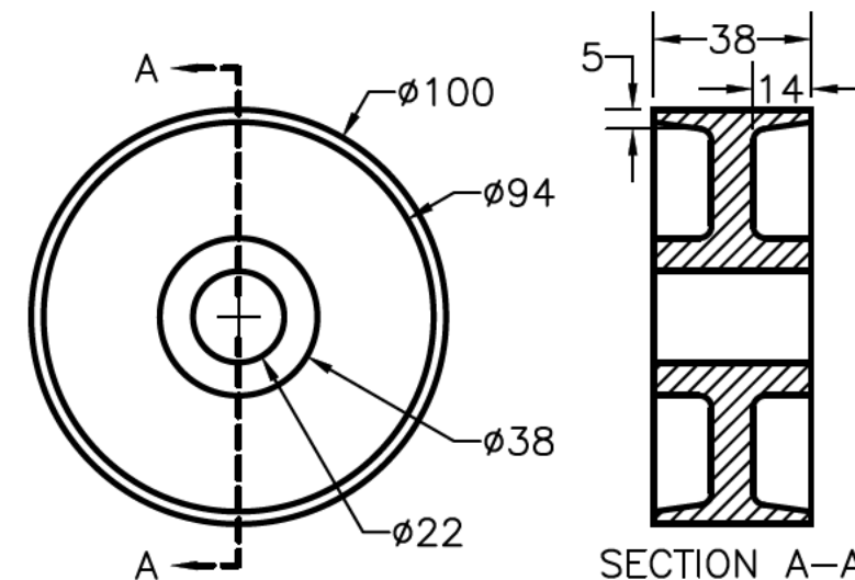
WHEEL SCALE 1:2
