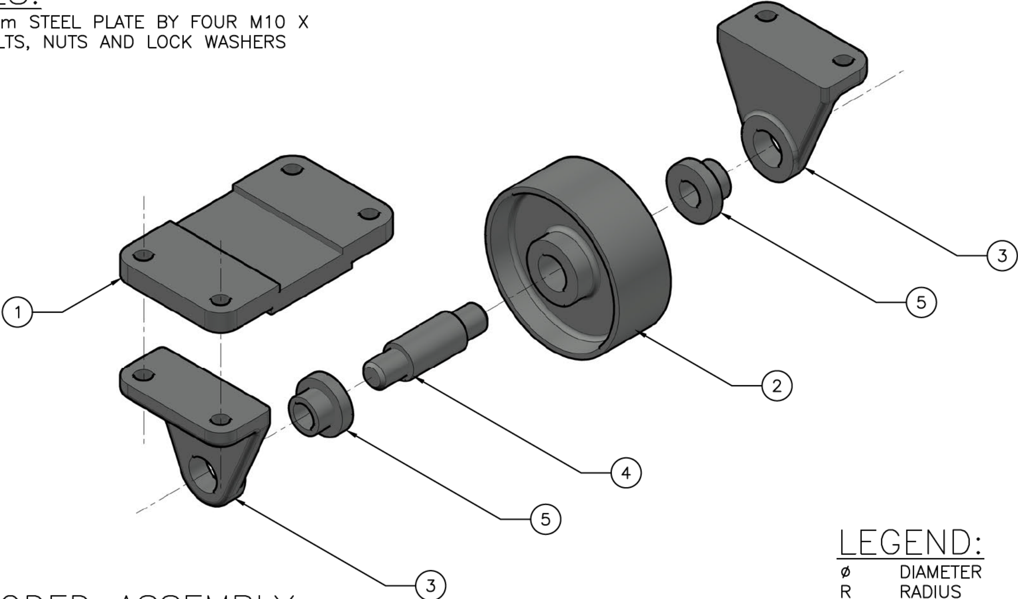
CASTER EXPLODED ASSEMBLY SCALE 1:2
