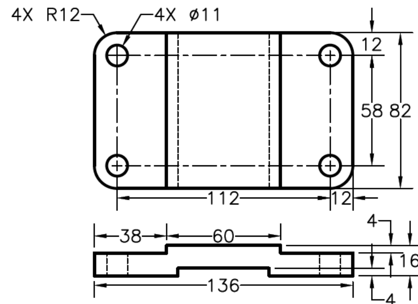
TOP PLATE SCALE 1:2
