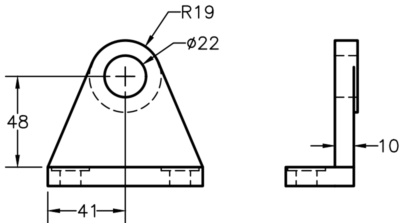
AXLE SUPPORT SCALE 1:2
