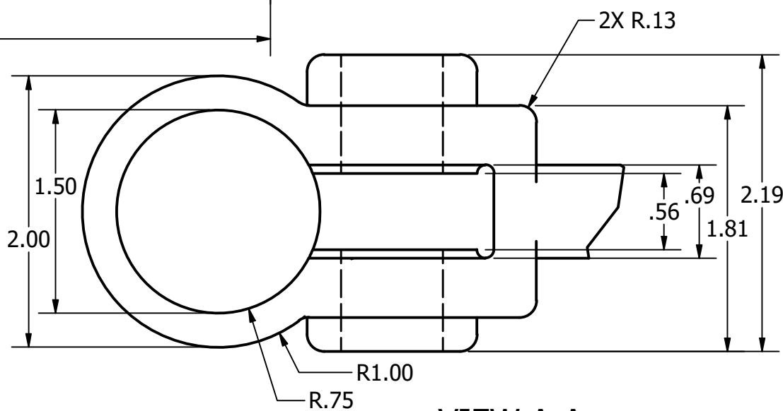
VIEW A-A SCALE 1 : 1
