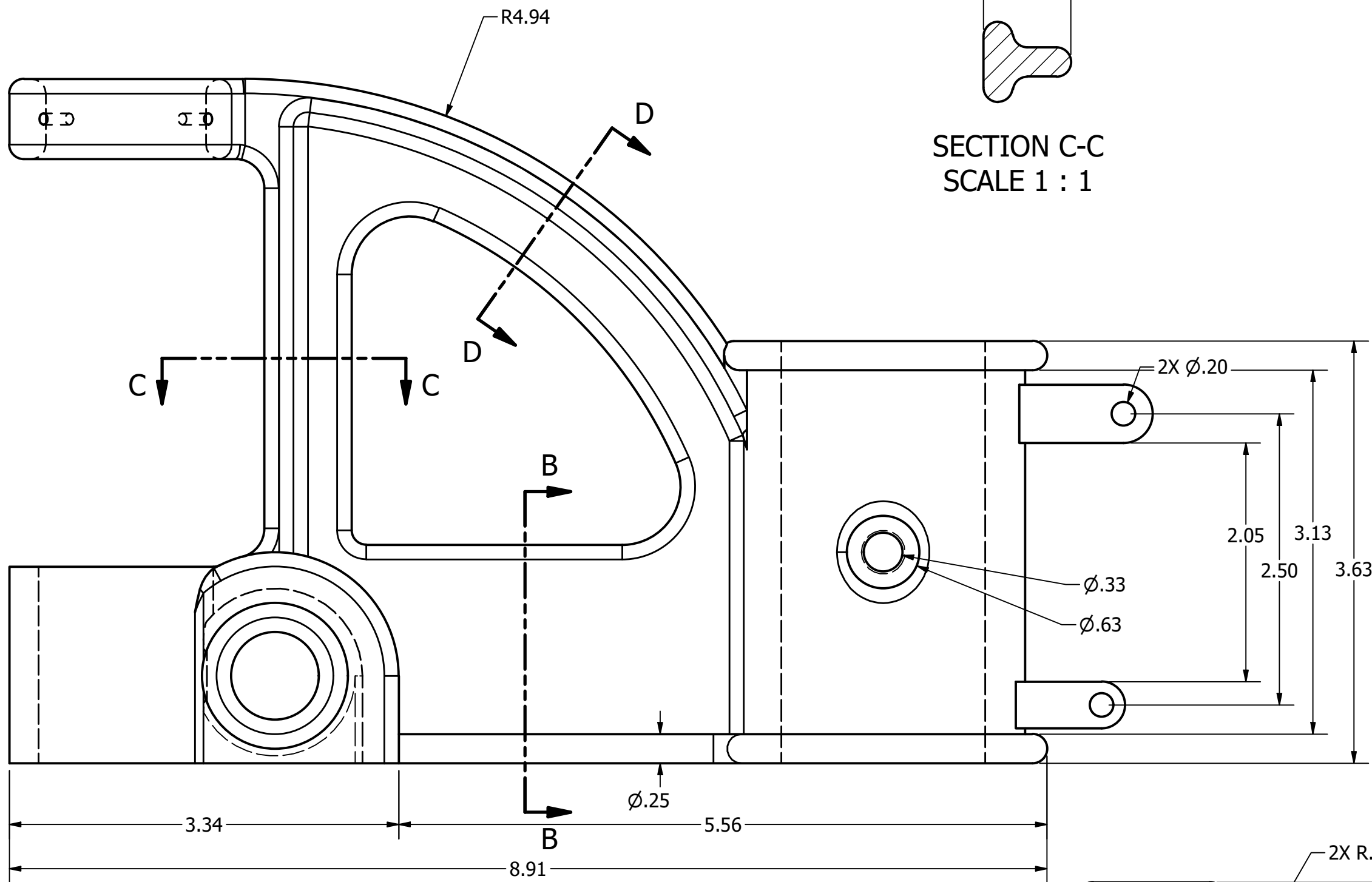
DRILL PRESS BRACKET SCALE 1 : 1
